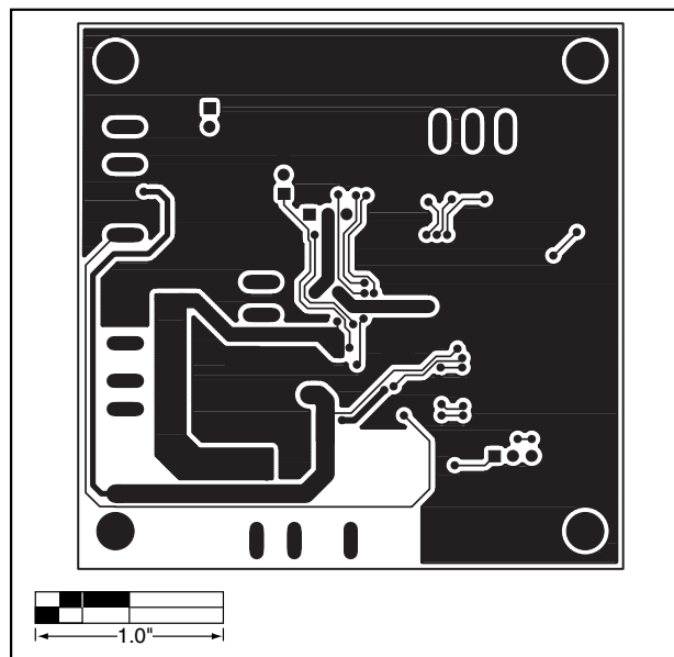
Figure 4. MAX1774 EV Kit PC Board Layout—Solder Side
