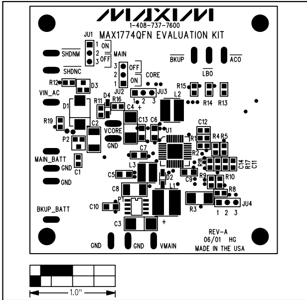
Figure 2. MAX1774 EV Kit Component Placement Guide—Component Side
