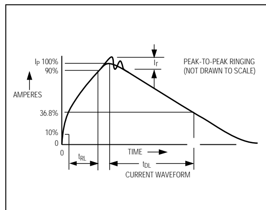
Figure 2b. Human Body Model Current Waveform
