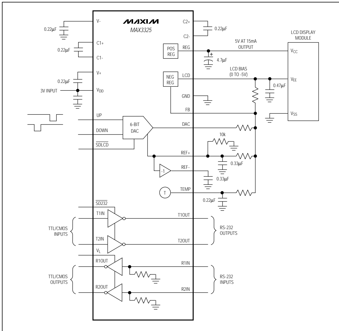
Typical Operating Circuit
