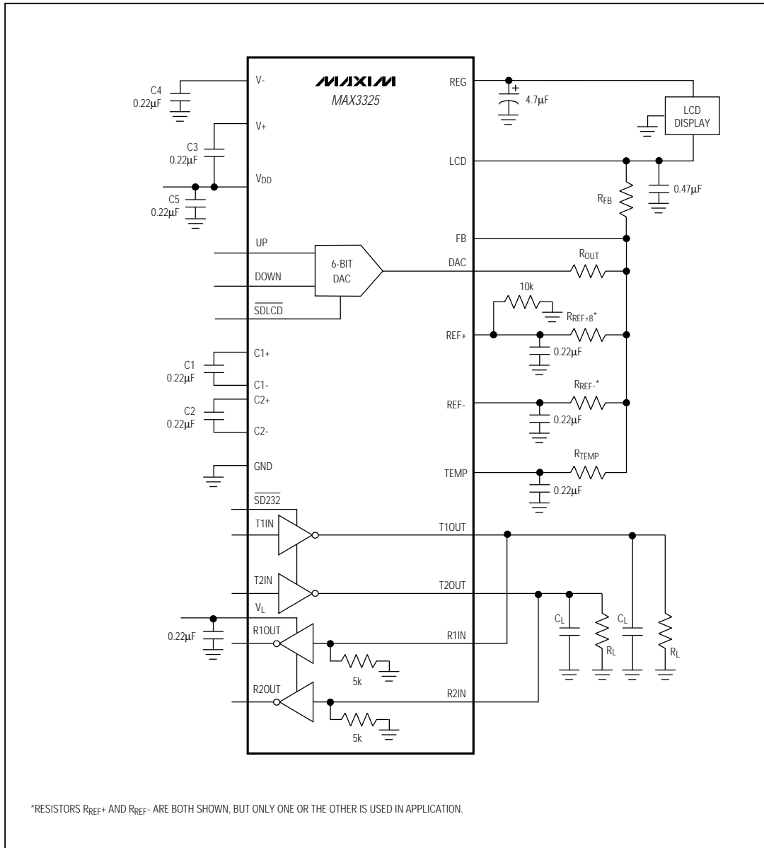
Figure 1. Application Circuit
