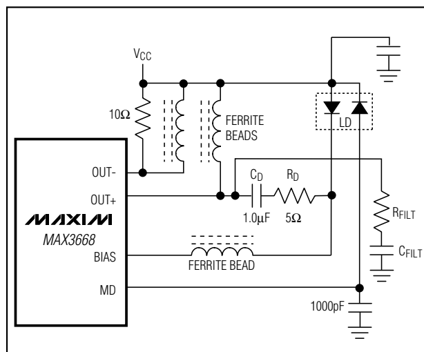
Figure 5. Output Termination for Maximum Modulation Current
