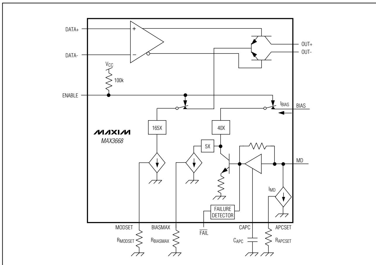
Figure 3. Functional Diagram
