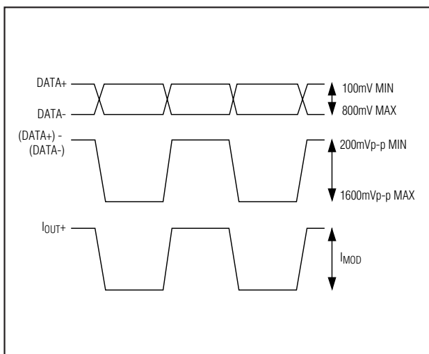
Figure 1. Required Input Signal and Output Polarity
