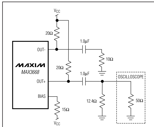
Figure 2. Output Termination for Characterization
