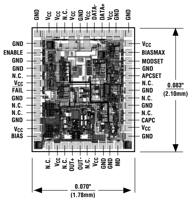
Chip Topography
