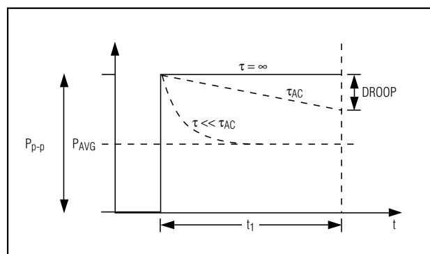
Figure 4. Droop
