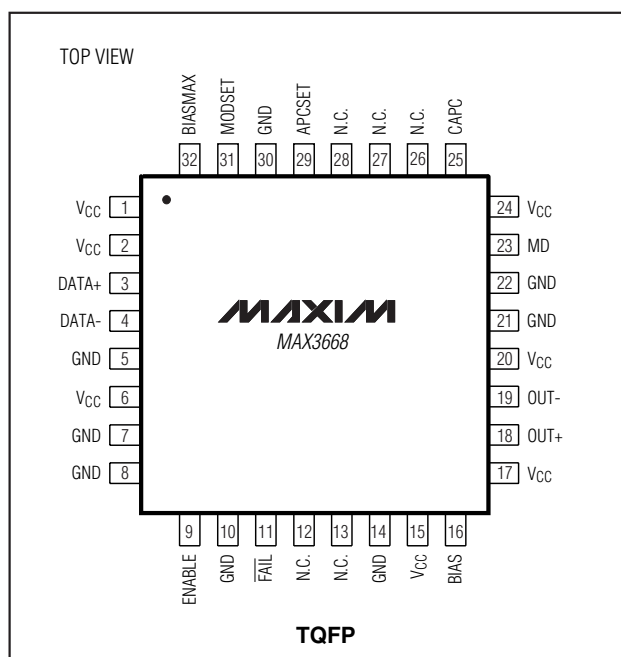
Pin Configuration
