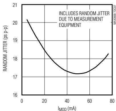
RANDOM JITTER vs. MODULATON CURRENT
