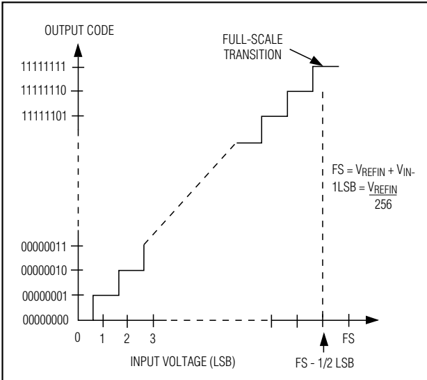
Figure 7. Input/Output Transfer Function
