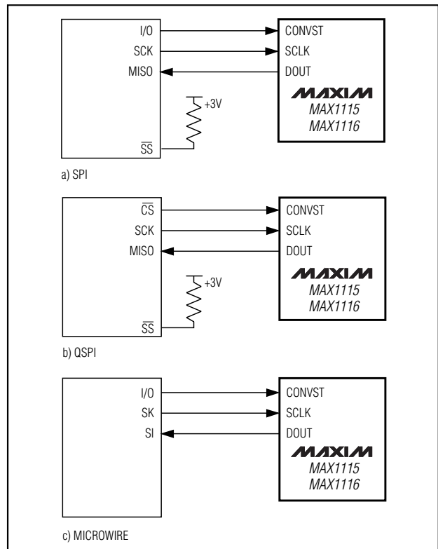
Figure 5. Common Serial-Interface Connections
