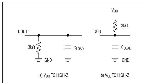
Figure 2. Load Circuits for Disable Time
