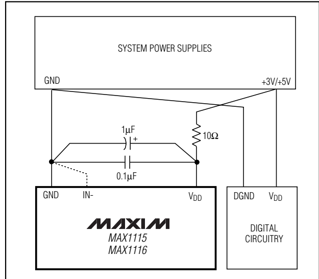
Figure 8. Power-Supply Connections
