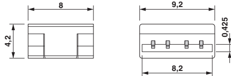
Dimensioned drawing
