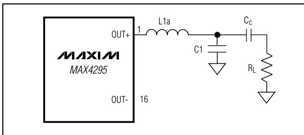
Figure 5. MAX4295 Single-Ended Configuration
