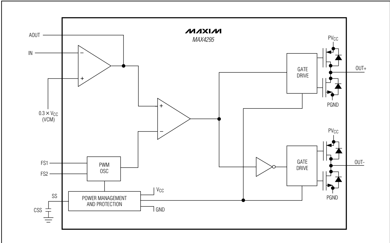
Figure 1. Functional Diagram
