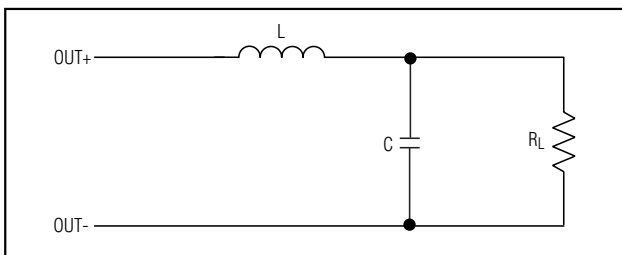
Figure 4a. Single-Ended 2-Pole Filter
