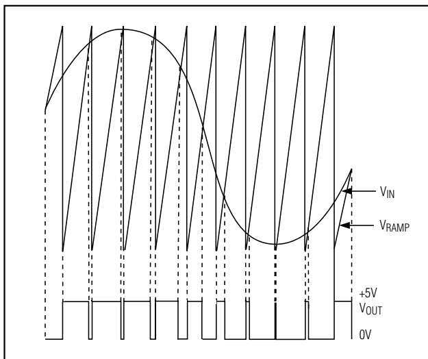
Figure 2. PWM Waveforms
