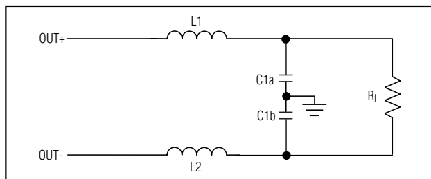
Figure 4b. Balanced 2-Pole Filter
