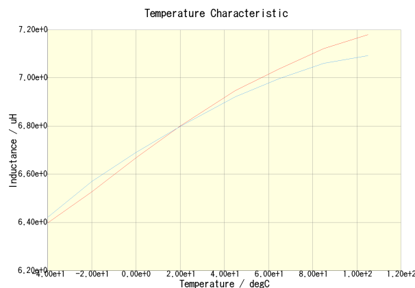
CLF6045T-6R8N-CA(DC = 0A)
