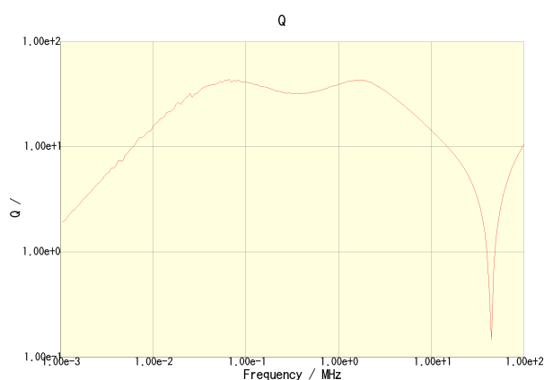
CLF6045T-6R8N-CA
