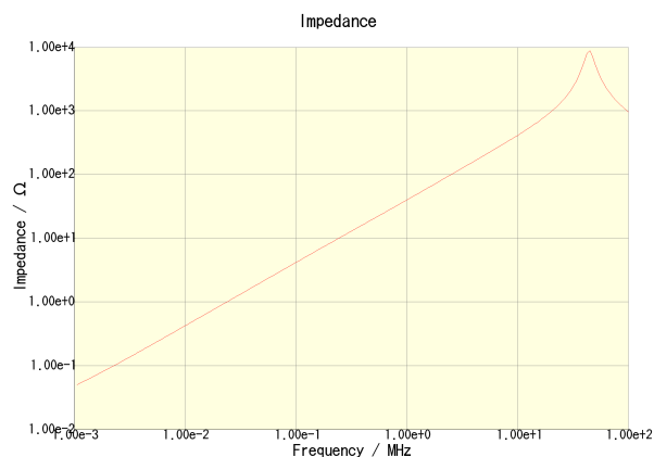
CLF6045T-6R8N-CA
