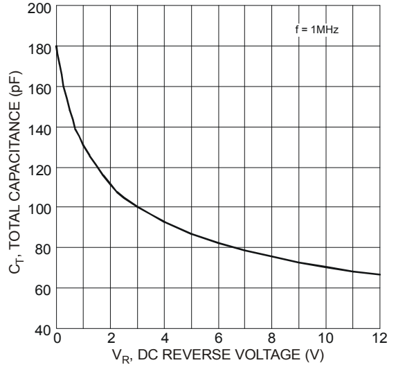
Figure 4 Typical Total Capacitance
