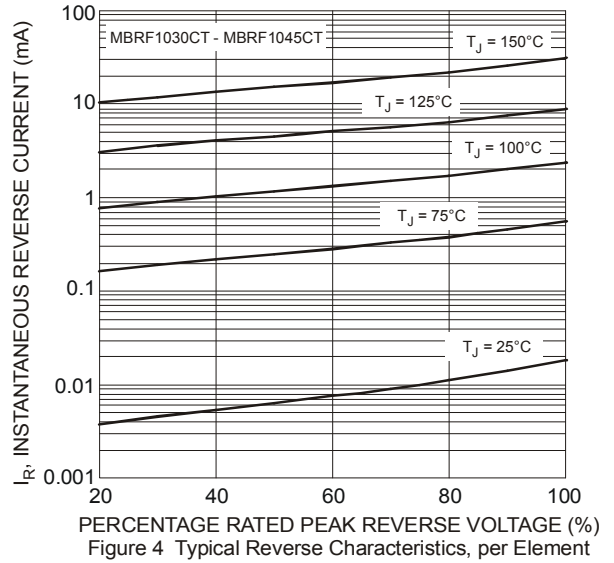
Figure 4 Typical Reverse Characteristics, per Element
