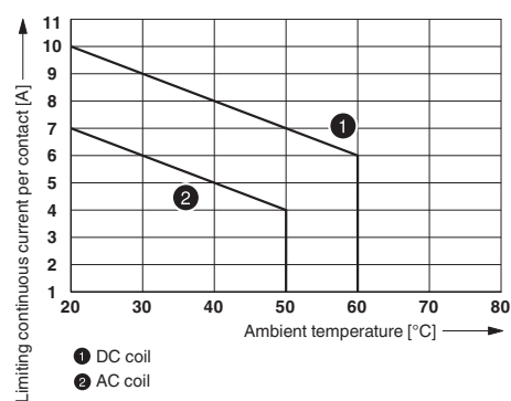
Contact derating
