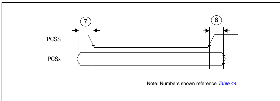
Figure 24. DSPI PCS strobe ( \overline{PCSS} ) timing
