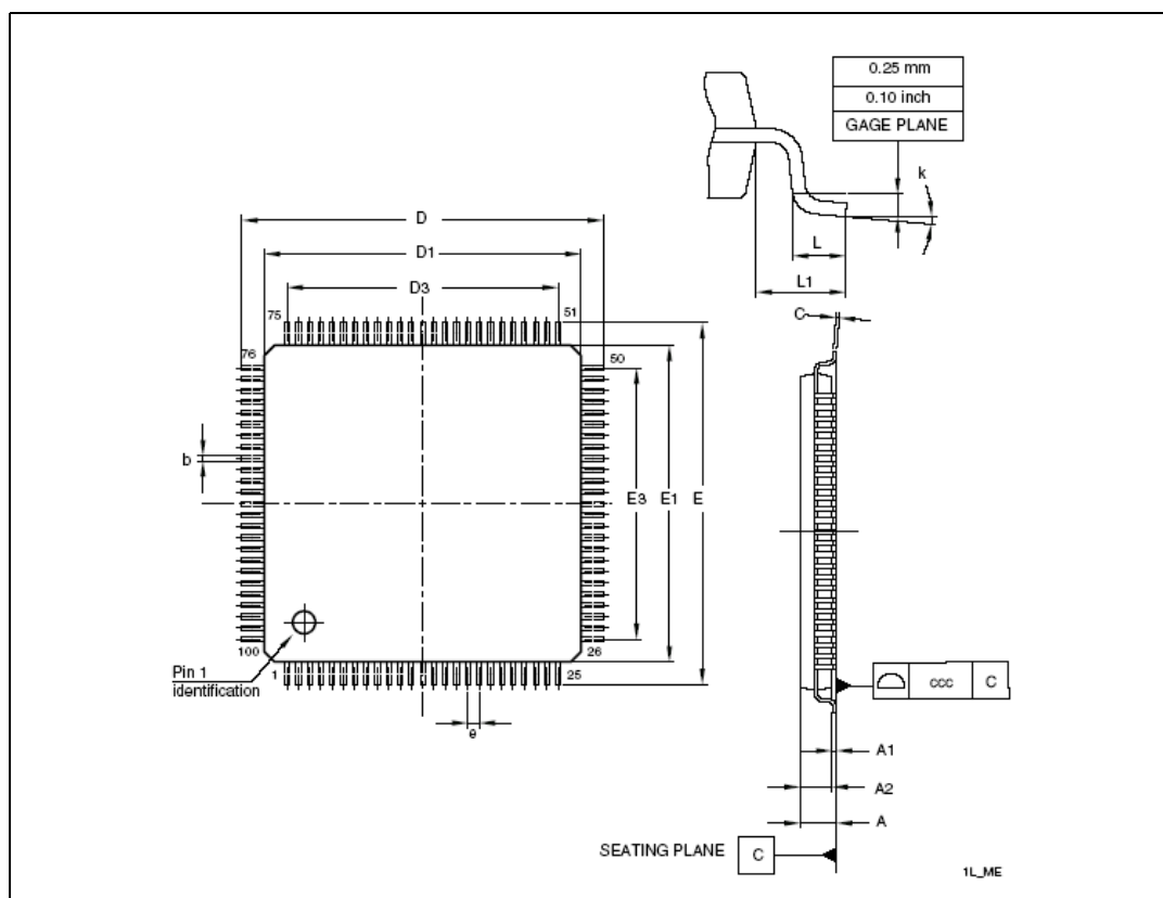
Figure 26. LQFP100 mechanical drawing
