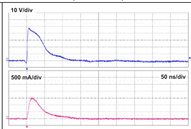
Figure 16. Response to ISO 7637-3 Pulse 3b (Us = +100 V)
