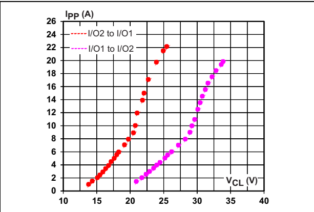
Figure 12. TLP measurements
