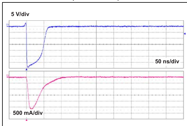
Figure 15. Response to ISO 7637-3 Pulse 3a (Us = -150 V)
