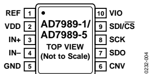
Figure 4. 10-Lead MSOP Pin Configuration
