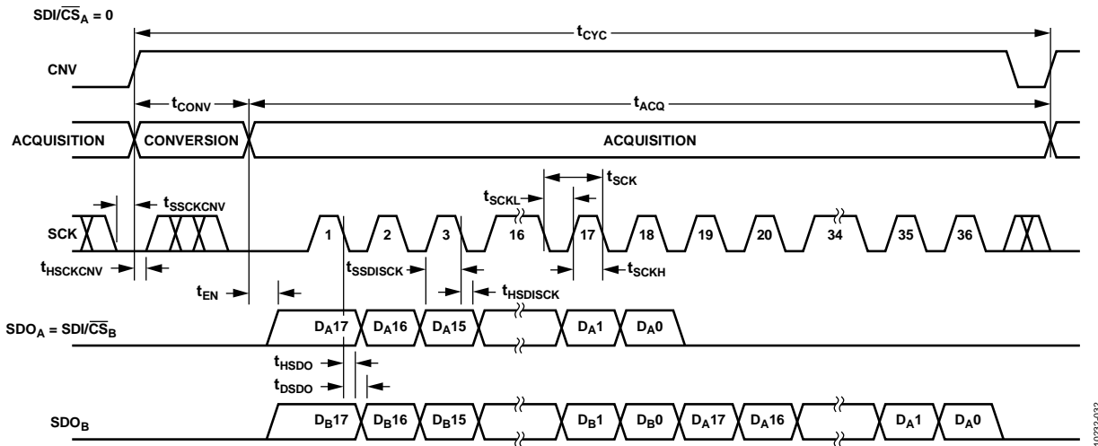
Figure 36. Chain Mode Serial Interface Timing
