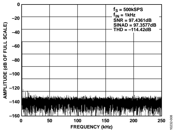
Figure 8. AD7989-5 FFT Plot
