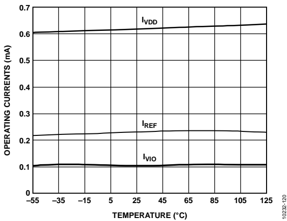
Figure 20. Operating Currents vs. Temperature (AD7989-5)
