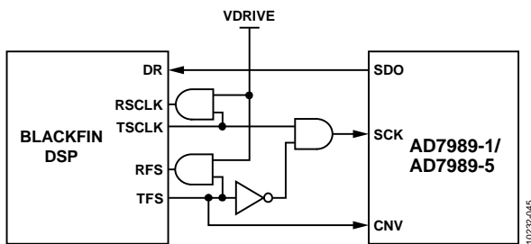
Figure 38. Evaluation Board Connection to Blackfin Sport Interface
