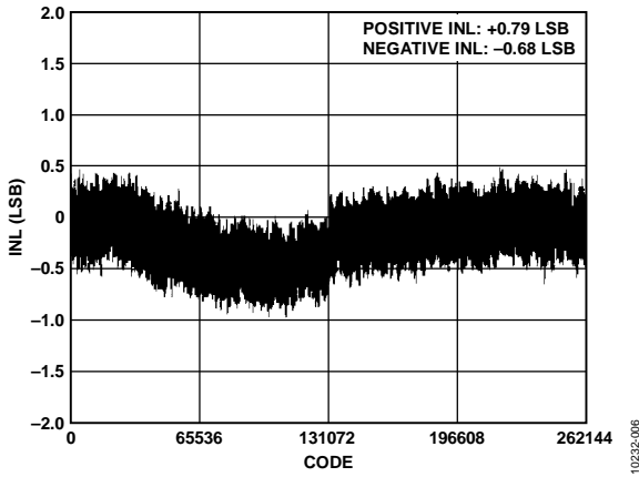
Figure 6. Integral Nonlinearity vs. Code
