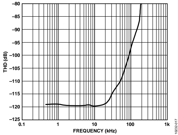
Figure 19. THD vs. Frequency
