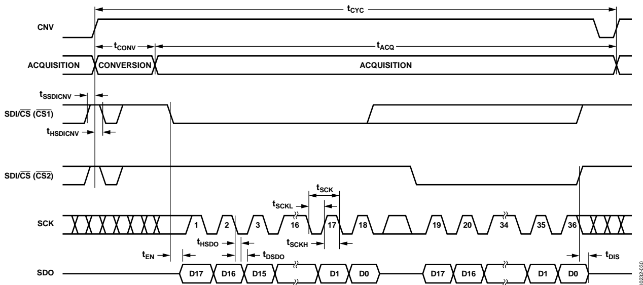
Figure 34. CS Mode, 4-Wire Serial Interface Timing
