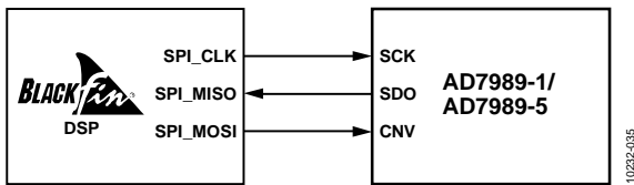
Figure 37. Typical Connection to Blackfin SPI Interface
