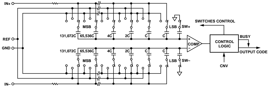
Figure 24. ADC Simplified Schematic
