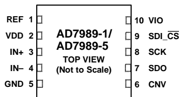
Figure 5. 10-Lead LFCSP Pin Configuration
