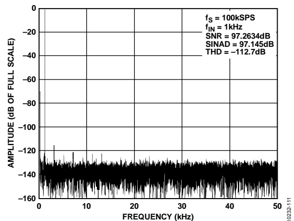
Figure 11. AD7989-1 FFT Plot
