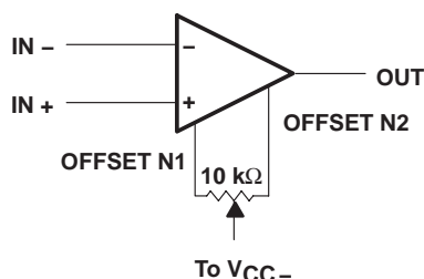
Figure 2. Input Offset Voltage Null Circuit
