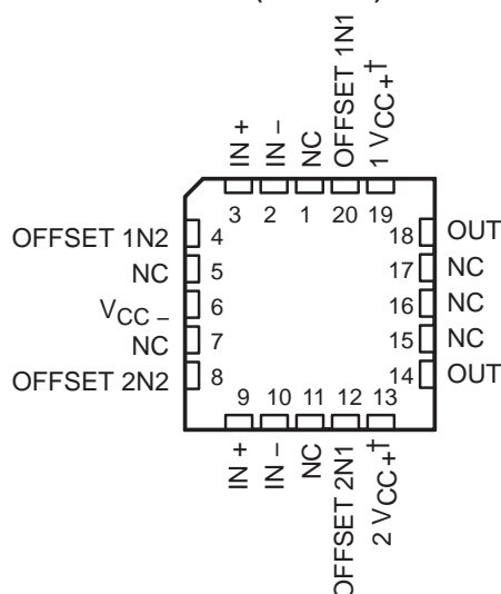
uA747m ... FK PACKAGE (TOP VIEW)
