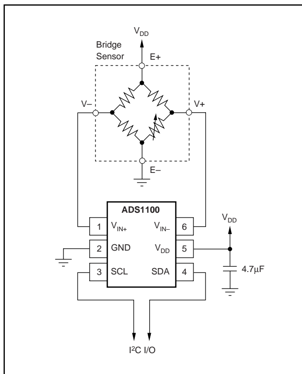
FIGURE 9. Measuring a Wheatstone Bridge Sensor.
