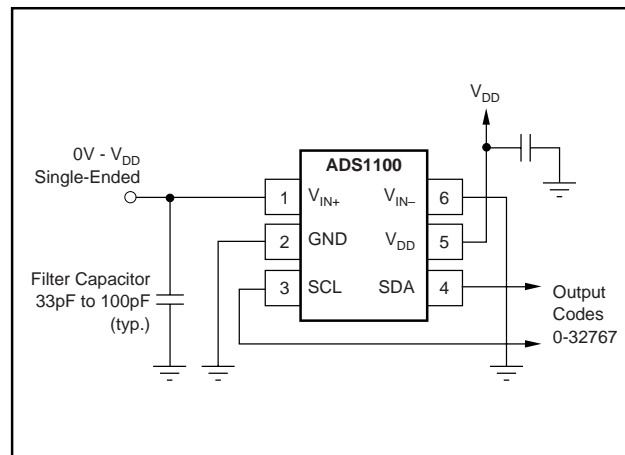
FIGURE 7. Measuring Single-Ended Inputs.
