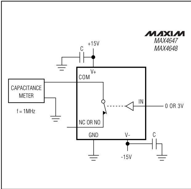
Figure 6. Channel-On Capacitance Test Circuit
