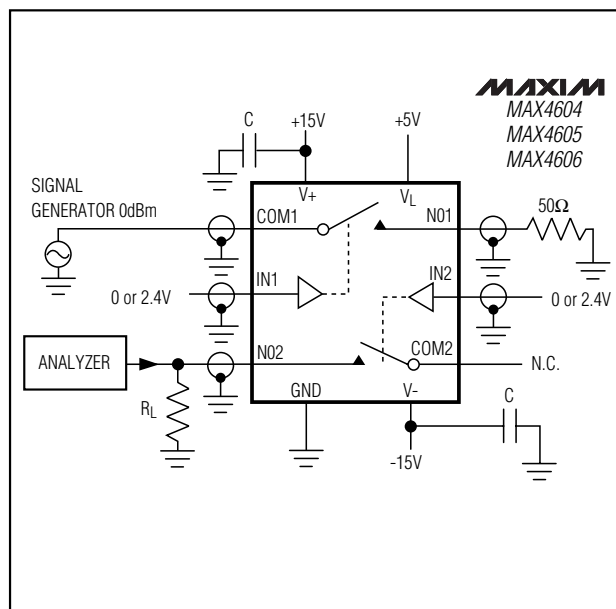
Figure 5. Crosstalk Test Circuit
