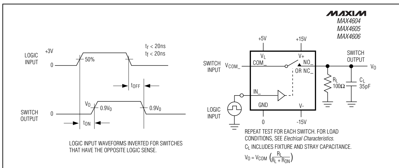
Figure 2. Switching-Time Test Circuit
