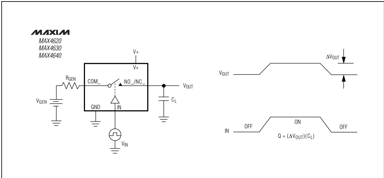
Figure 4. Charge Injection
