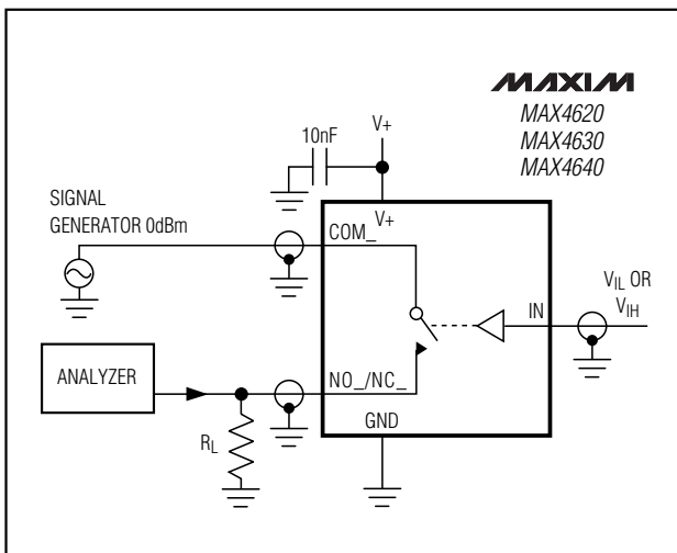
Figure 2. Off-Isolation/On-Channel Bandwidth
