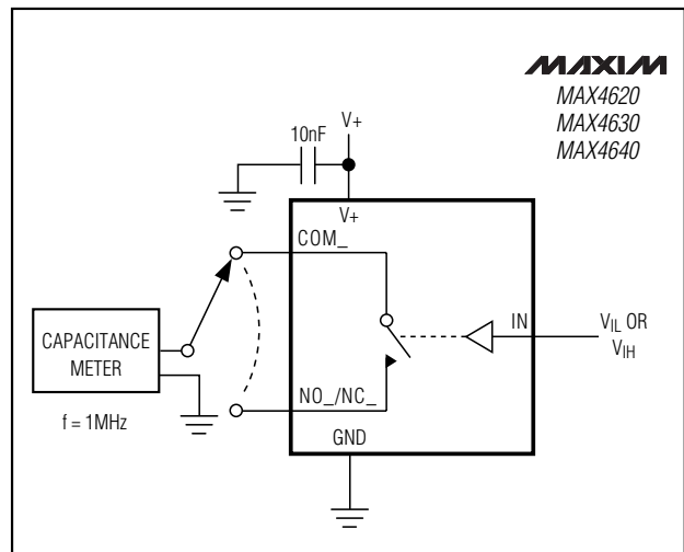
Figure 3. Channel Off/On-Capacitance
