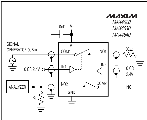
Figure 5. Crosstalk
