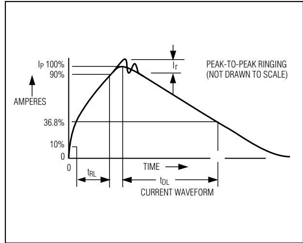
Figure 7. Human Body Model Current Waveform
