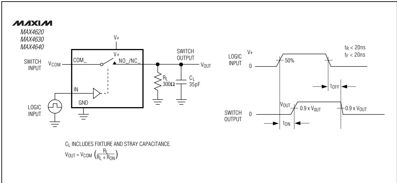
Figure 1. Switching Time
