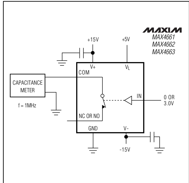
Figure 8. Switch On-Capacitance Test Circuit
