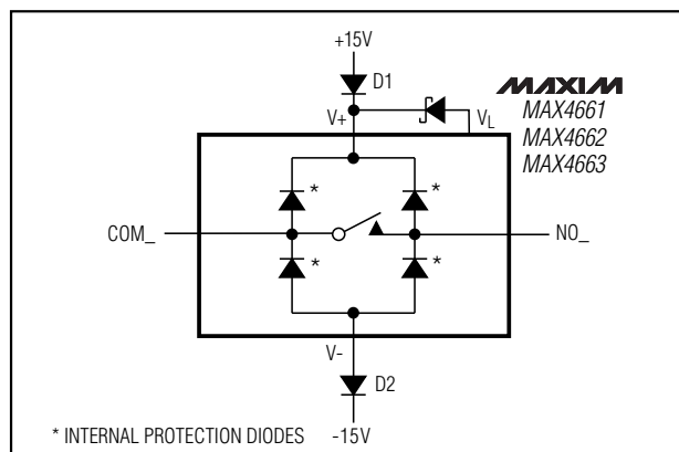
Figure 1. Overvoltage Protection Using External Blocking Diodes
