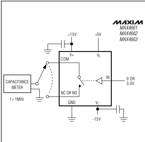
Figure 7. Switch Off-Capacitance Test Circuit
