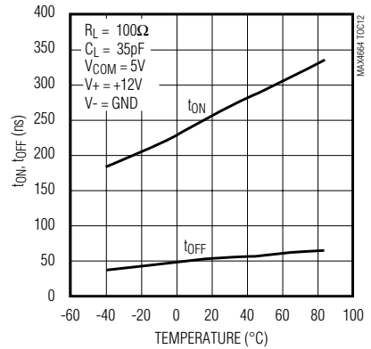
ON/OFF TIMES vs. TEMPERATURE (SINGLE SUPPLY)
