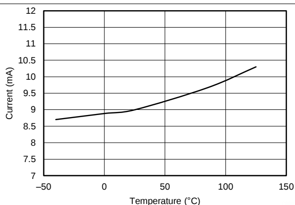
Figure 1. I_{VDD0} Charging Current vs. Temperature
