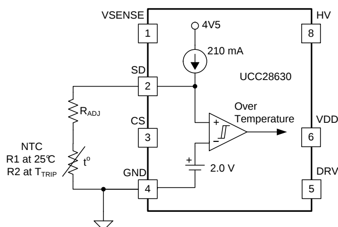
Figure 37. Fault Interface to SD Pin
