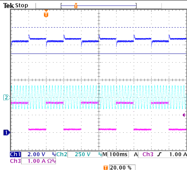
Figure 58. Transient Step 5% to 50% Load, 115 V AC
