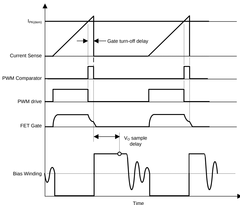
Figure 25. V_{OUT} Sample Adjust for External Gate Delay
