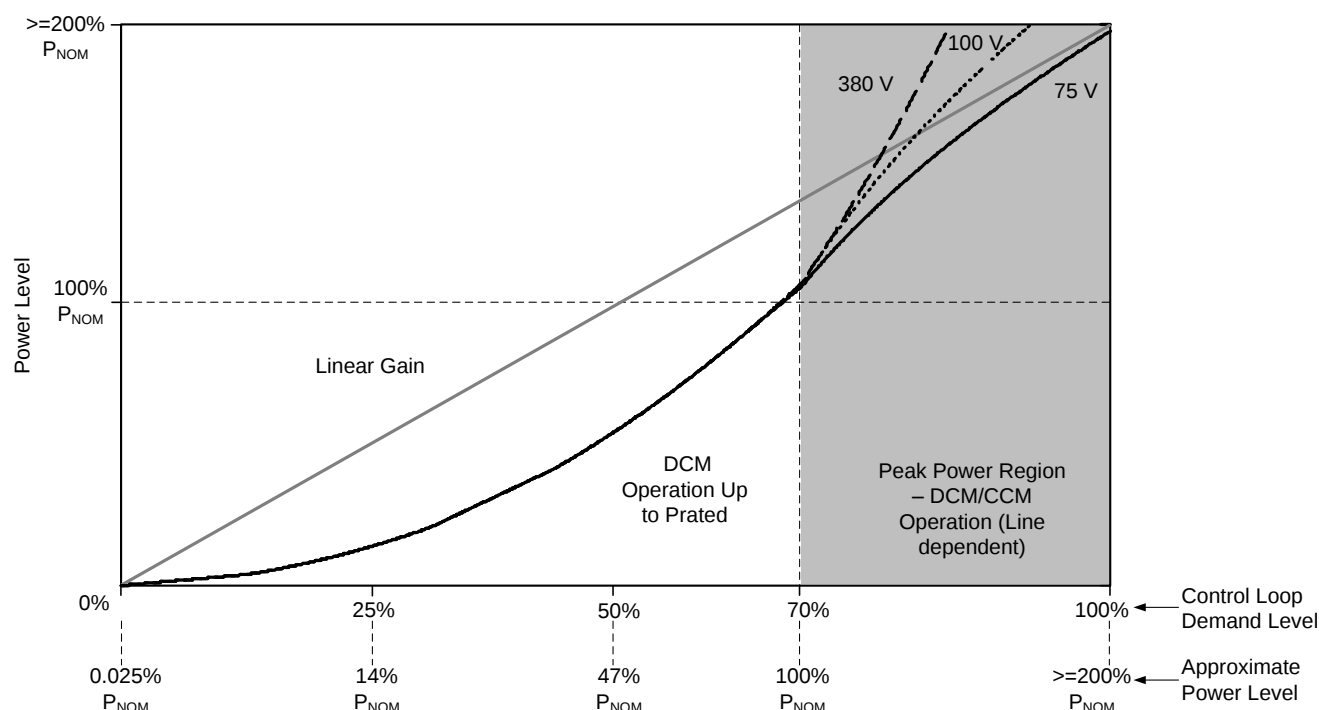
Figure 42. Modulator Gain Curves vs Bulk Capacitor Voltage
