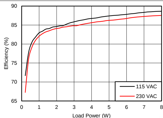
Figure 54. Zoom Light-Load Efficiency vs. Load/Line (cable drop included)
