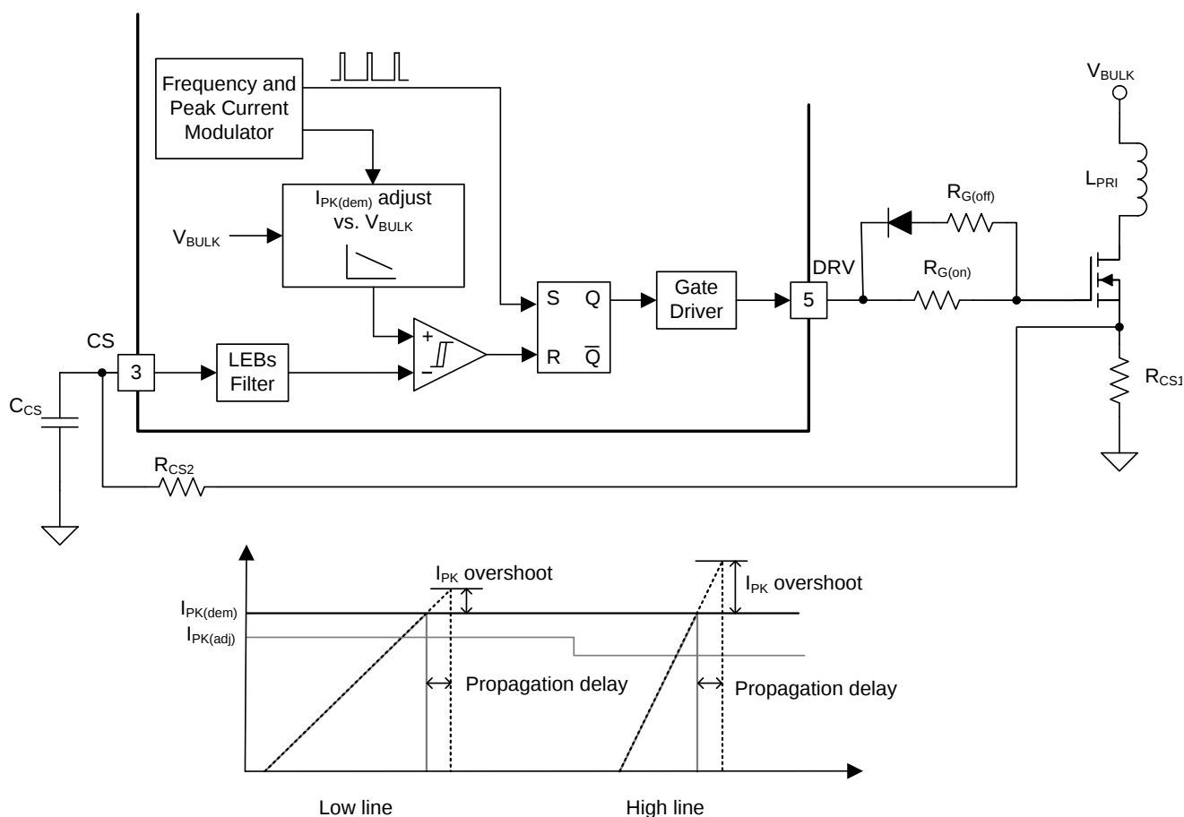
Figure 32. Peak-Current Demand Adjustment vs V_{BULK} to Correct Prop Delay Overshoot
