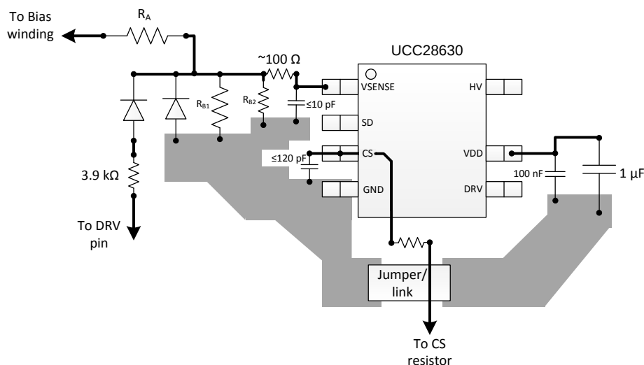
Figure 63. Recommended PCB Layout for Single-Sided Assembly
