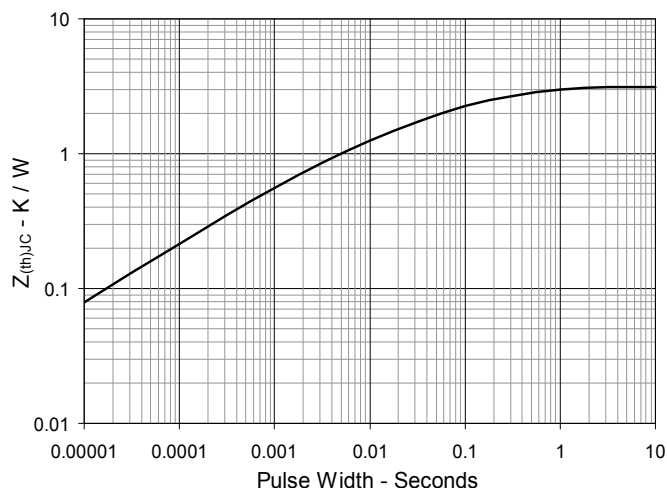
Fig. 8. Maximum Transient Thermal Resistance
