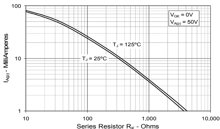
Fig. 2. Plateau Current vs. External Resistance
