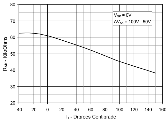
Fig. 7. Dynamic Resistance vs. Junction Temperature
