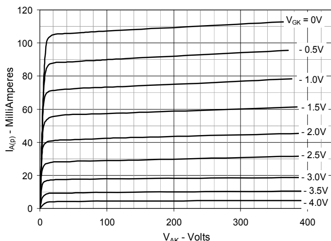
Fig. 6. Extended Output Curves @ T_J = 125^\circ\text{C}
