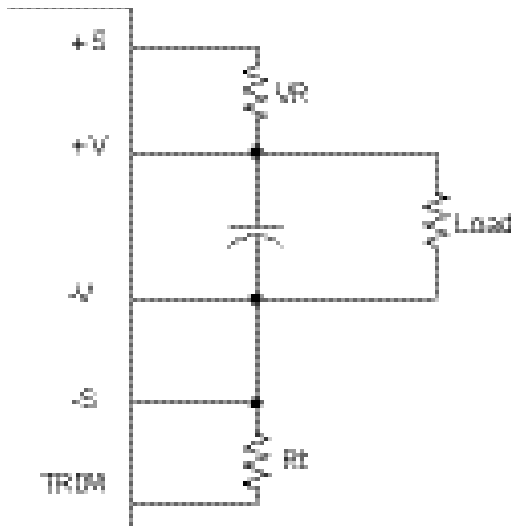
Figure 2 External Resistors
