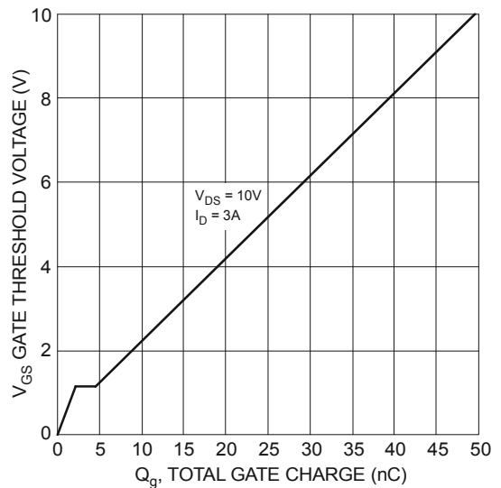
Figure 10 Gate Charge
