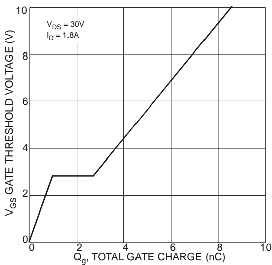
Figure 11 Gate Charge
