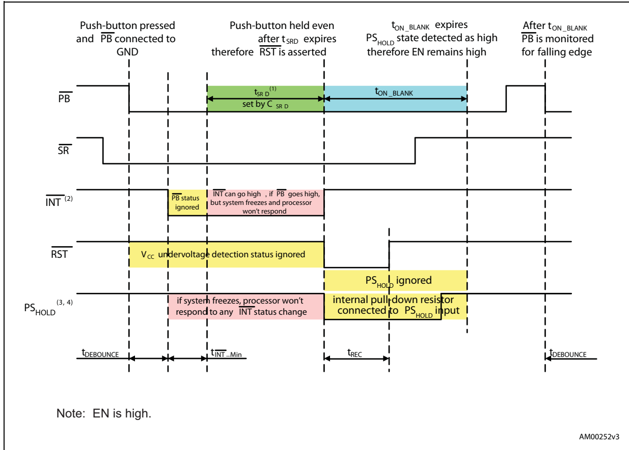
Figure 18. Long push (option with RST assertion)
