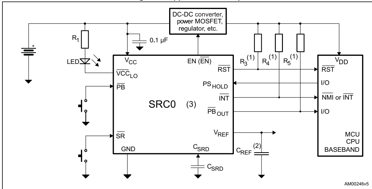
Figure 1. Application hookup
