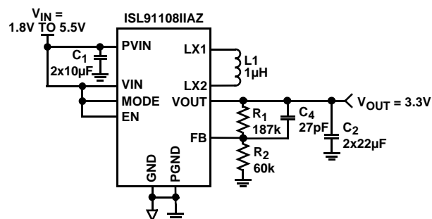
FIGURE 4. TYPICAL ISL91108IAZ APPLICATION
