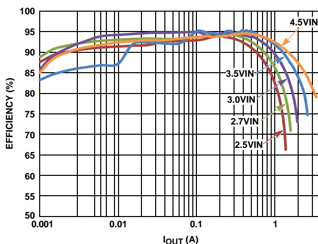
FIGURE 2. ISL91108IINZ EFFICIENCY vs OUTPUT CURRENT
