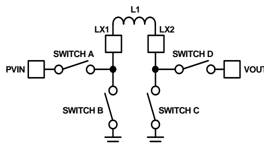
FIGURE 3. BUCK-BOOST TOPOLOGY
