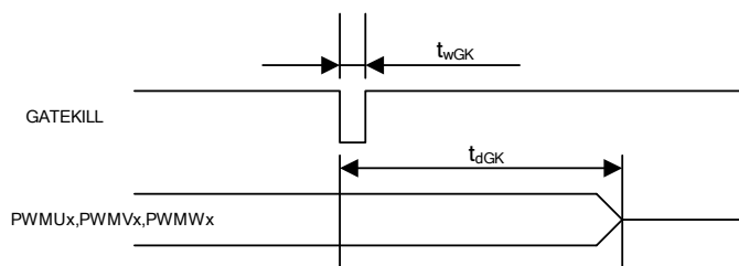
Figure 6 Gatekill timing
