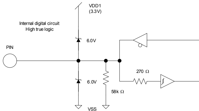
Figure 16 PWMUL/PWMUH/PWMVL/PWMVH/PWMWL/PWMWH output
