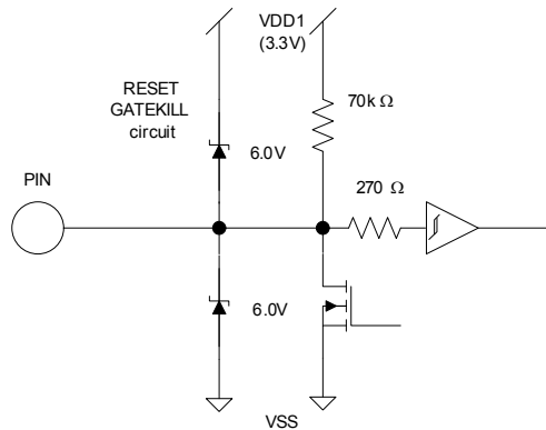
Figure 18 RESET, GATEKILL I/O
