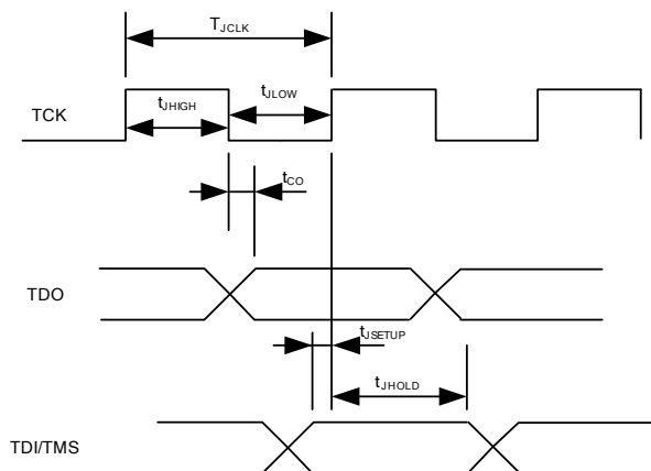
Figure 15 JTAG timing
