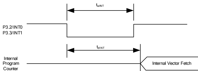
Figure 8 Interrupt timing
