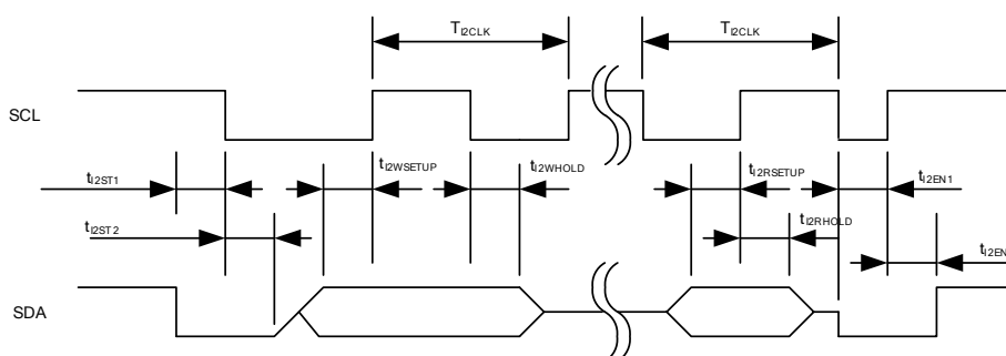
Figure 9 I 2 C Timing
