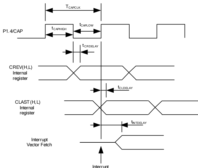
Figure 13 CAPTURE timing
