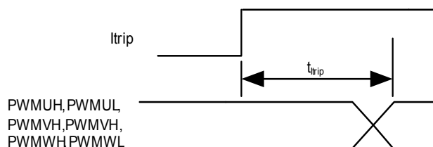
Figure 7 ITRIP timing
