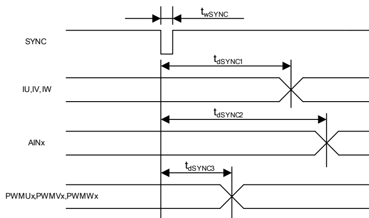
Figure 5 SYNC timing
