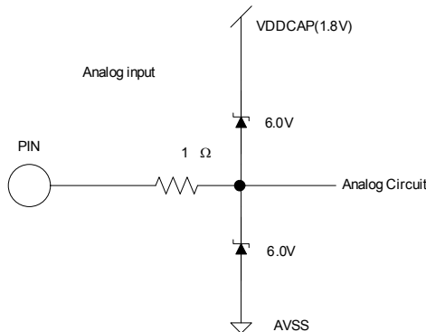
Figure 19 Analog input
