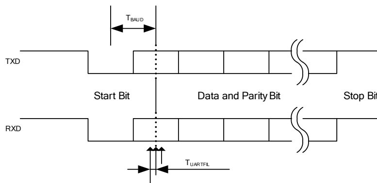
Figure 12 UART timing
