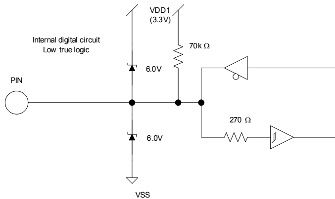
Figure 17 All digital I/O except motor PWM output
