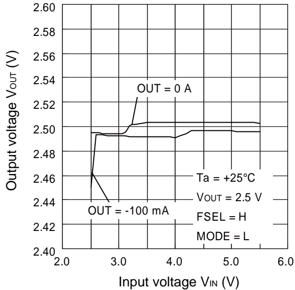
Output voltage vs. Input voltage (3.2 MHz: PFM/PWM mode)
