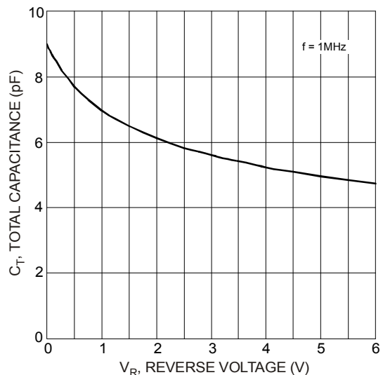
Figure 2 Total Capacitance
