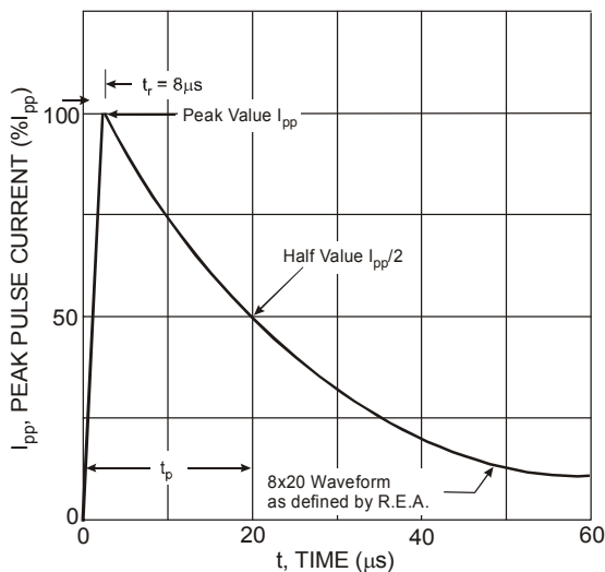
Figure 1 Pulse Waveform
