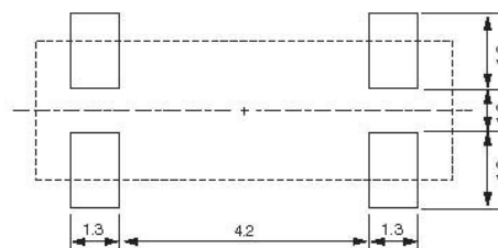
Figure 2) Bottom View and Suggested Land
