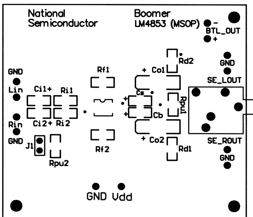
Figure 40. Recommended MM PC Board Layout: Component-Side SilkScreen
