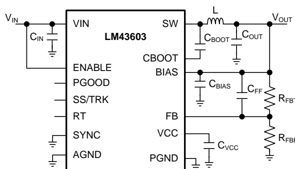
Figure 46. LM43603 Basic Schematic for V OUT ≥ 3.3 V, tie BIAS to V OUT
