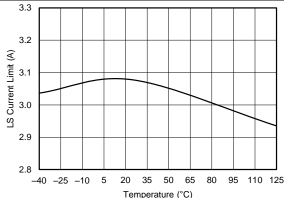
Figure 26. Low-Side Current Limit vs Junction Temperature
