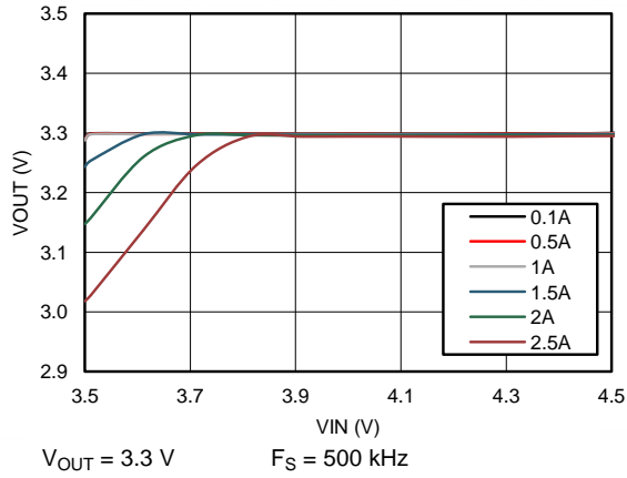
Figure 61. Dropout Curve
