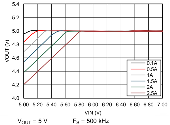
Figure 76. Drop-out Curve
