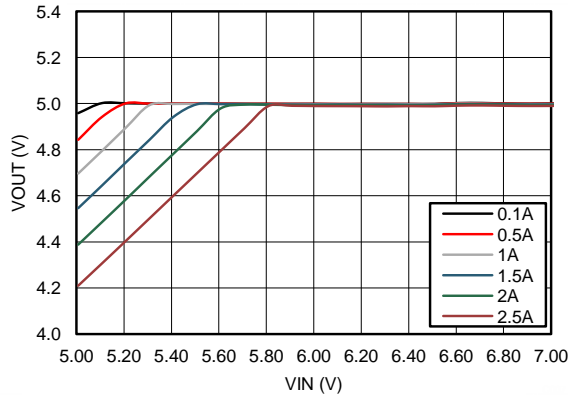
Figure 13. Dropout Curve
