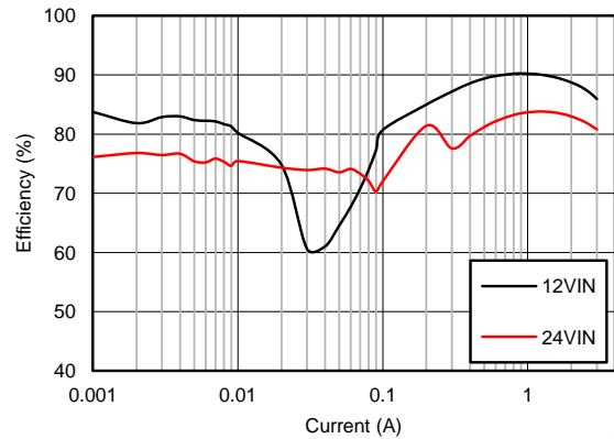
Figure 80. Efficiency
