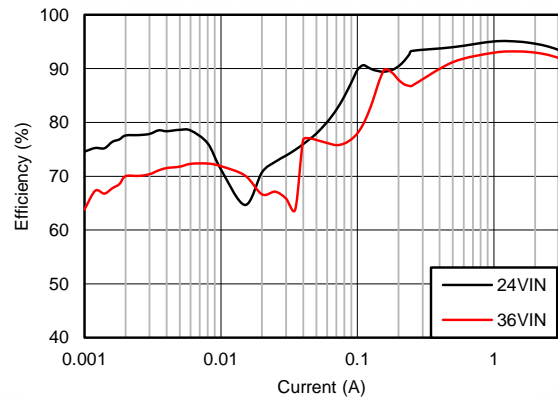
Figure 92. Efficiency
