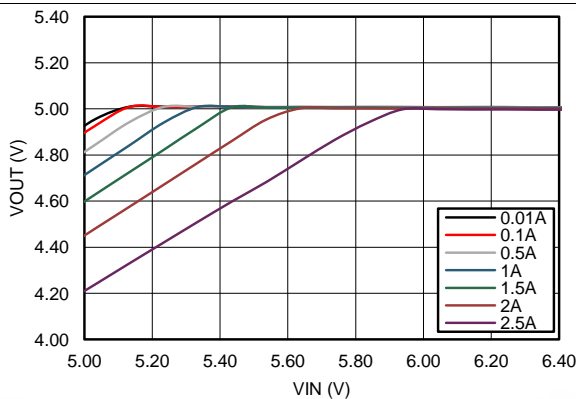
Figure 15. Dropout Curve
