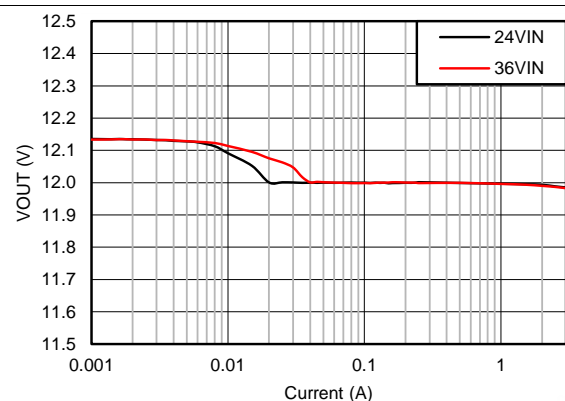
V_{OUT} = 12\text{ V} F_S = 500\text{ kHz}
