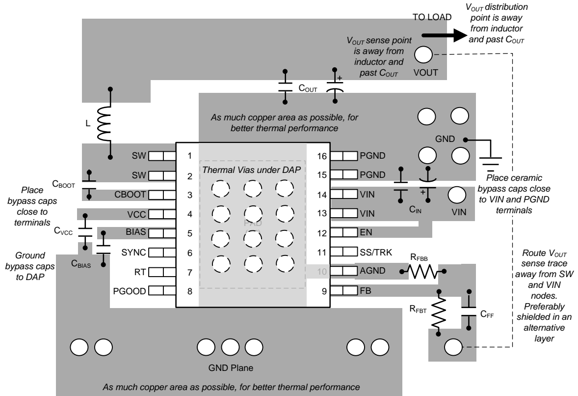
Figure 99. LM43603 Board Layout Recommendations
