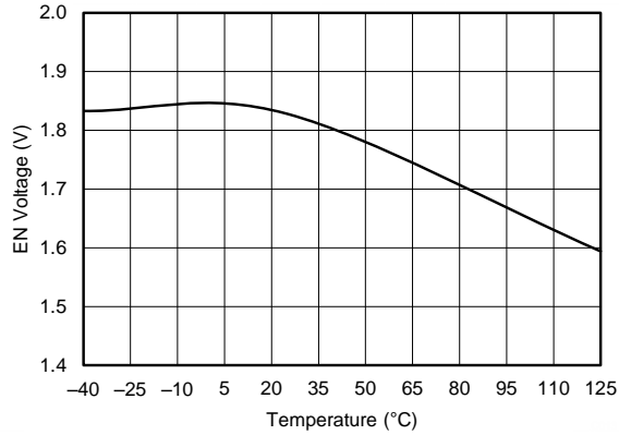
Figure 19. EN Falling Threshold
