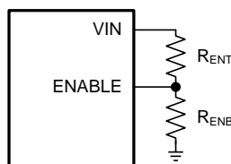
Figure 37. System UVLO By Enable Dividers
