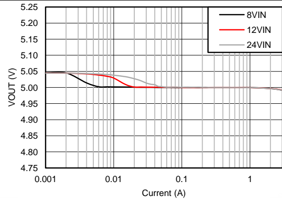
V_{OUT} = 5\text{ V} F_S = 200\text{ kHz}
