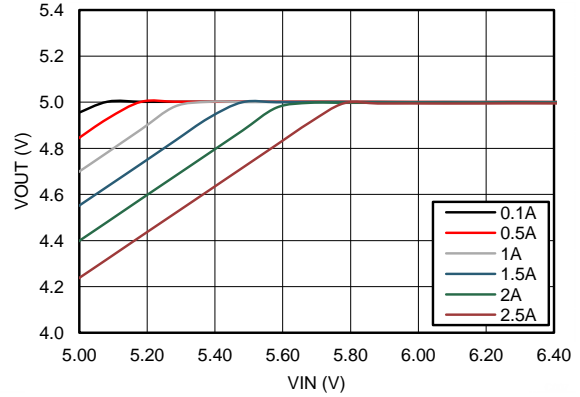
Figure 14. Dropout Curve
