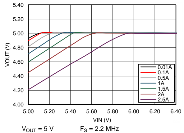
Figure 88. Drop-out Curve
