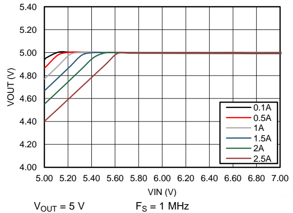
Figure 82. Drop-out Curve
