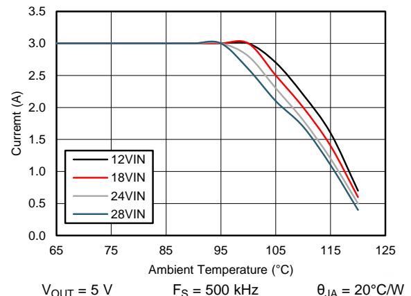
Figure 78. Derating Curve
