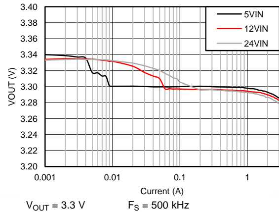
Figure 64. Output Voltage Regulation
