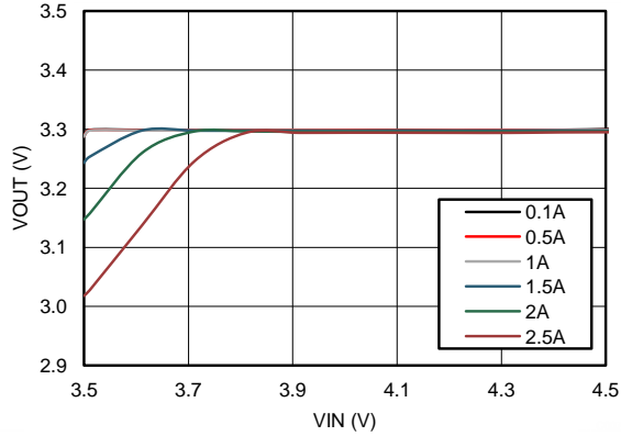
Figure 13. Dropout Curve
