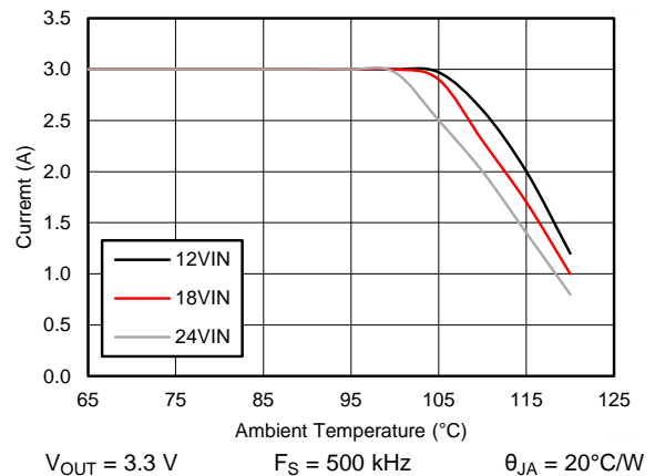
Figure 66. Derating Curve
