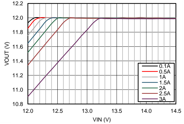
Figure 94. Drop-out Curve
