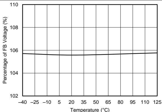
Figure 27. PGOOD OVP Falling Threshold vs Junction Temperature
