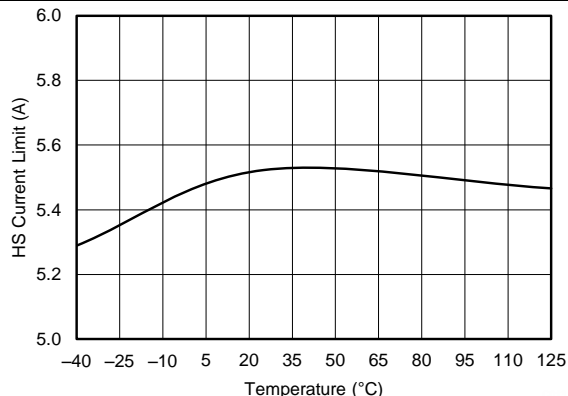
Figure 25. High-Side Current Limit vs Junction Temperature
