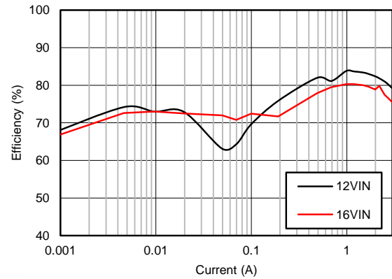
Figure 86. Efficiency
