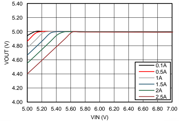
Figure 14. Dropout Curve
