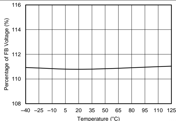
Figure 28. PGOOD OVP Rising Threshold vs Junction Temperature
