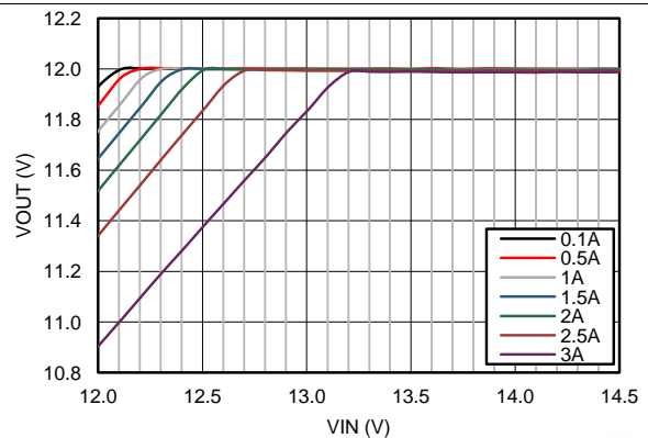
Figure 16. Dropout Curve
