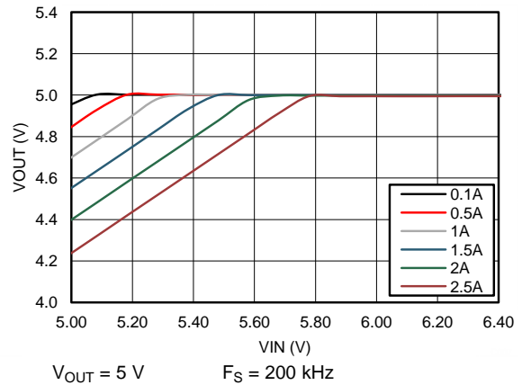
Figure 70. Drop-out Curve
