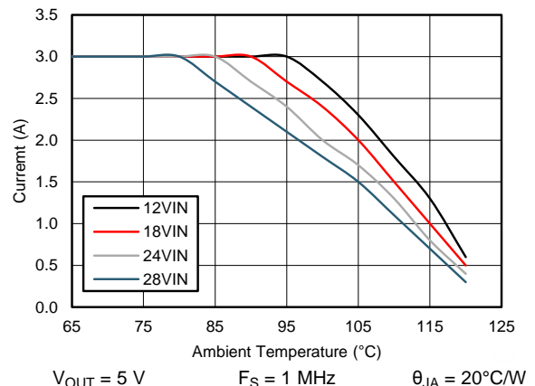
Figure 84. Derating Curve
