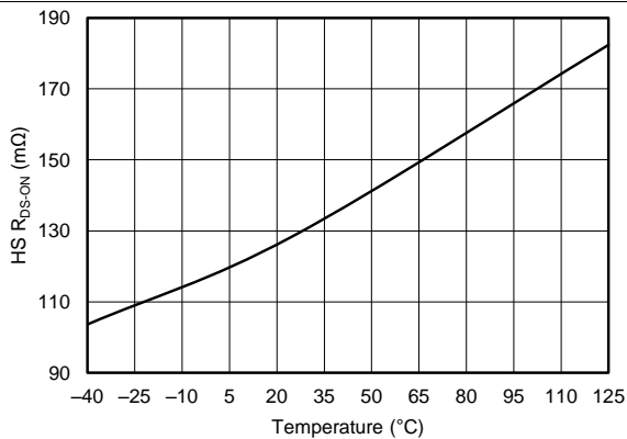
Figure 23. High-Side FET On Resistance vs Junction Temperature
