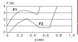
FORCE/TRAVEL DIAGRAM
