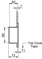
sectional drawing A-A
