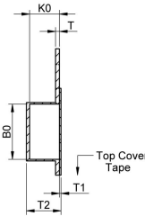
sectional drawing A-A
