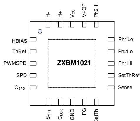
U-QFN4040-20
