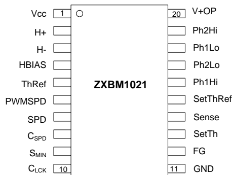
QSOP-20
