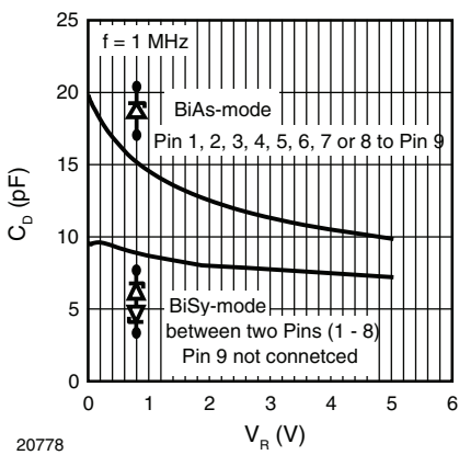
Fig. 3 - Typical Capacitance C_D vs. Reverse Voltage V_R
