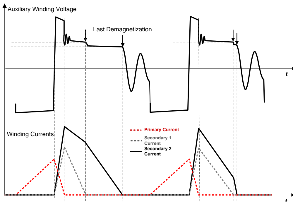
Figure 48. Winding Current Waveform in Multi-Output Flyback Converter
