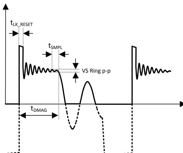
Figure 22. VS Voltage
