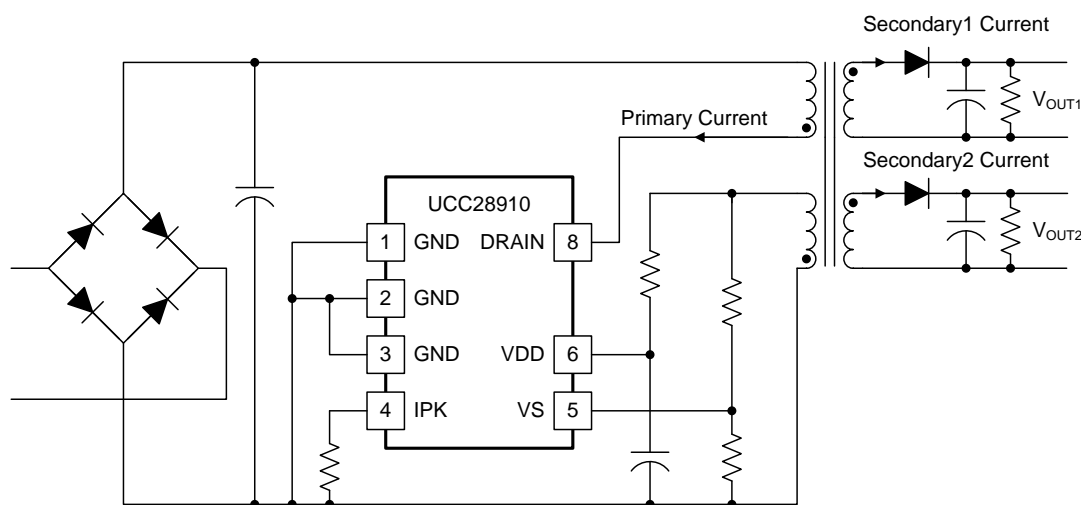
Figure 47. Multi-Output Flyback Converter
