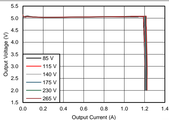
Figure 39. Output V-I Characteristic
