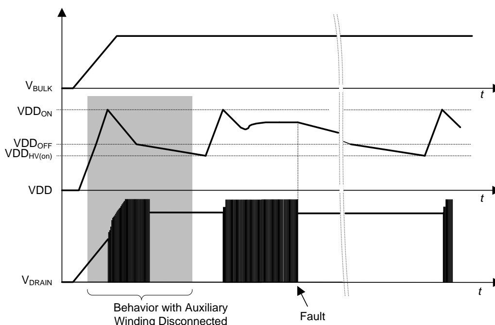
Figure 30. Start Up and Auto Re-Start Operation
