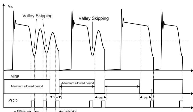
Figure 28. Valley Skipping
