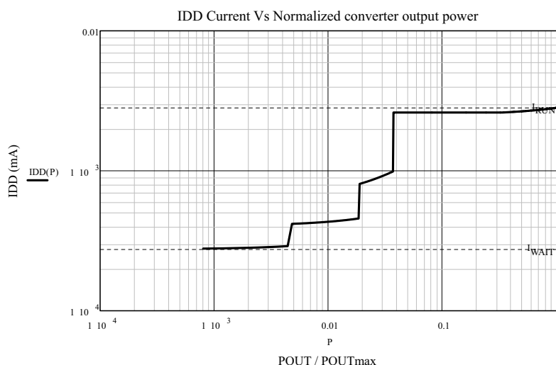
Figure 1. VDD Current Consumption
