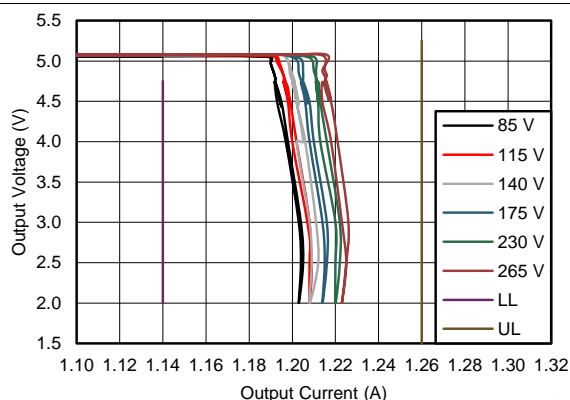
Figure 41. Output V-I Characteristic Output Voltage Regulation
