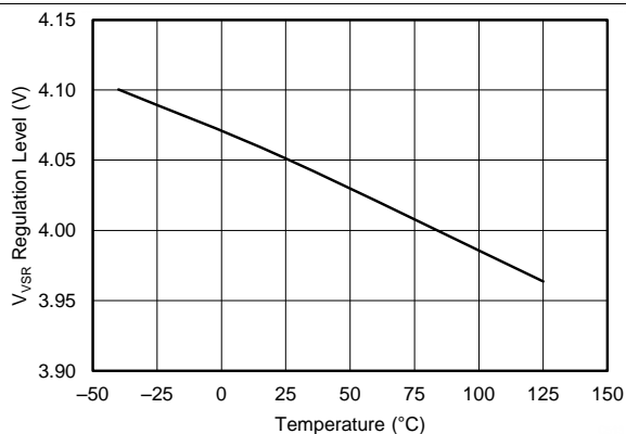
Figure 14. V_{VSR} vs Temperature
