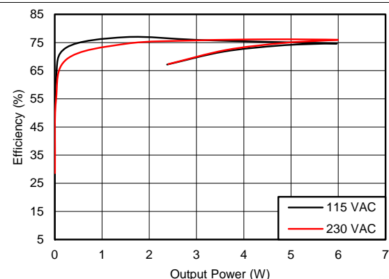
Figure 42. Efficiency vs P_{OUT} Diagram
