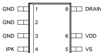
Pin Functions
