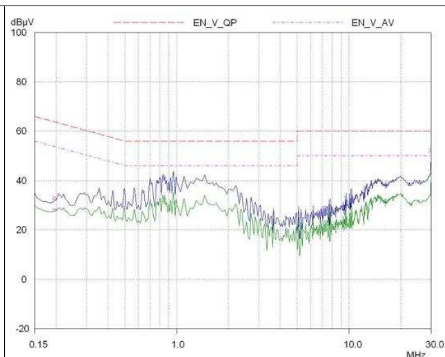
Figure 46. EMI Test Results per EN55022, Class B. 230-V AC Input
