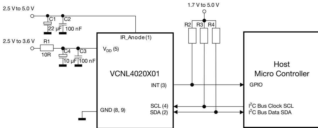
Fig. 12 - Application Circuit (x) = Pin Number
