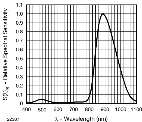
Fig. 7 - Relative Spectral Sensitivity vs. Wavelength (Proximity Sensor)
