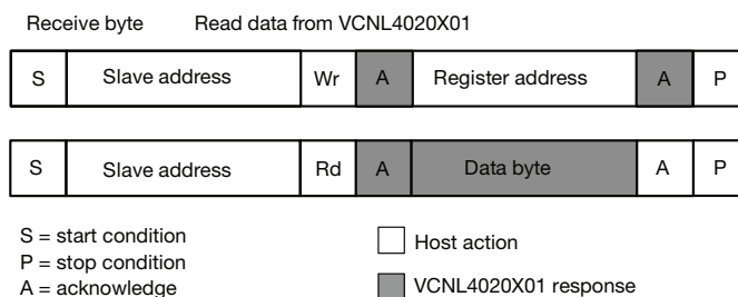
Fig. 14 - Send Byte/Receive Byte Protocol
