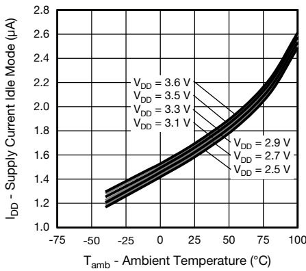
Fig. 1 - Idle Current vs. Ambient Temperature
