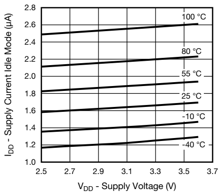
Fig. 2 - Idle Current vs. V DD
