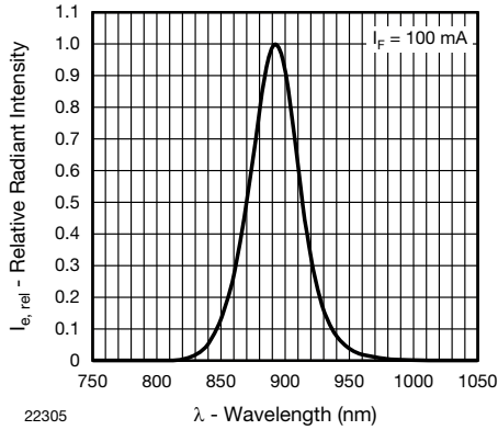
Fig. 5 - Relative Radiant Intensity vs. Wavelength
