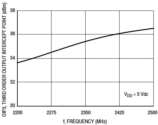
Figure 33. Third Order Output Intercept Point versus Frequency
