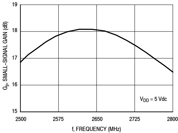
Figure 13. Small-Signal Gain (S21) versus Frequency
