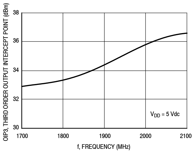
Figure 25. Third Order Output Intercept Point versus Frequency
