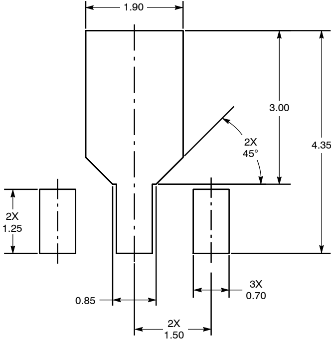
Figure 51. PCB Pad Layout for SOT-89A
