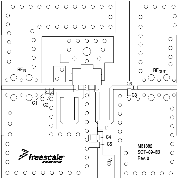
Figure 3. MMG20241HT1 Test Circuit Component Layout
