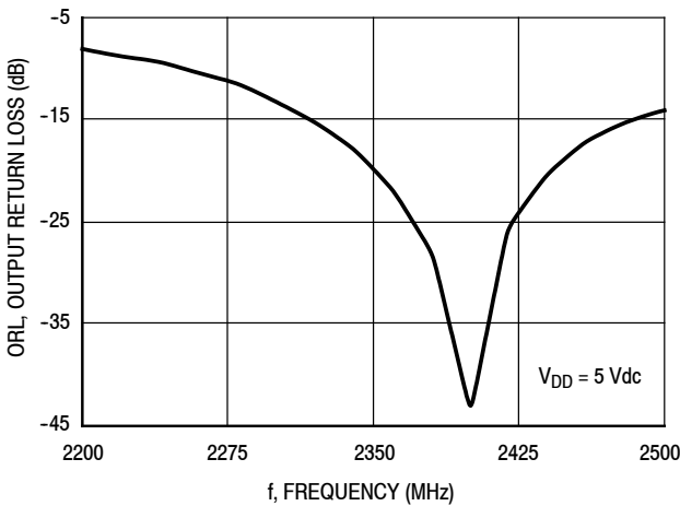
Figure 31. Output Return Loss (S22) versus Frequency
