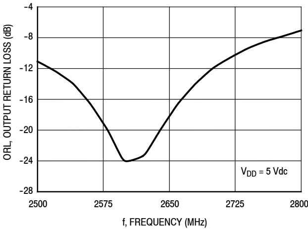
Figure 15. Output Return Loss (S22) versus Frequency
