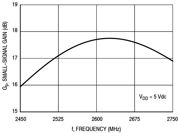
Figure 37. Small-Signal Gain (S21) versus Frequency
