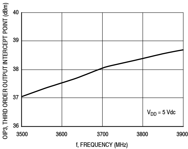
Figure 49. Third Order Output Intercept Point versus Frequency
