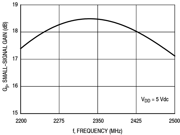
Figure 29. Small-Signal Gain (S21) versus Frequency
