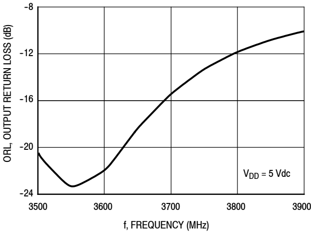
Figure 47. Output Return Loss (S22) versus Frequency
