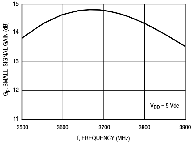
Figure 45. Small-Signal Gain (S21) versus Frequency
