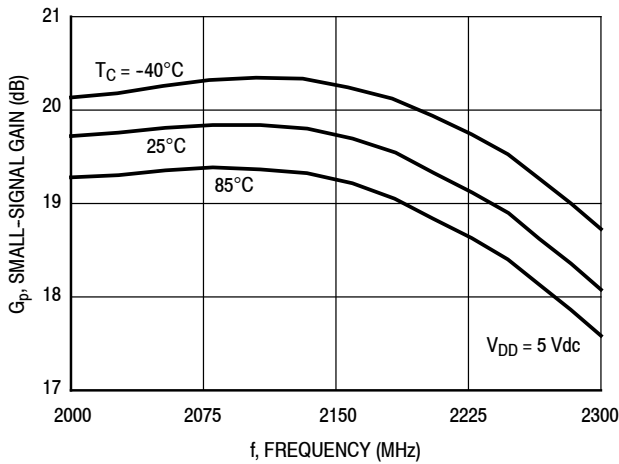
Figure 4. Small-Signal Gain (S21) versus Frequency versus Temperature
