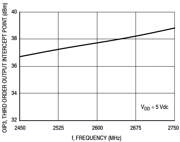
Figure 41. Third Order Output Intercept Point versus Frequency
