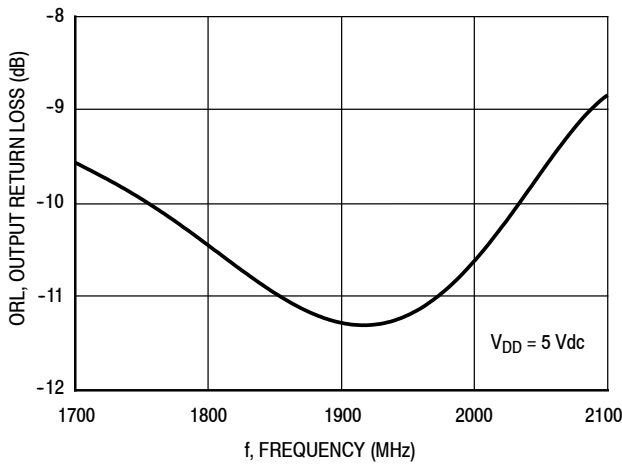
Figure 23. Output Return Loss (S22) versus Frequency
