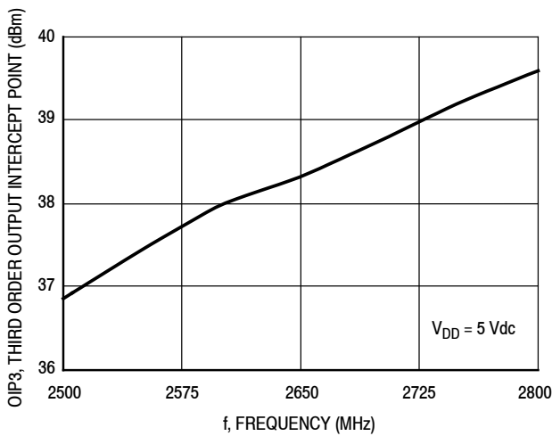
Figure 17. Third Order Output Intercept Point versus Frequency
