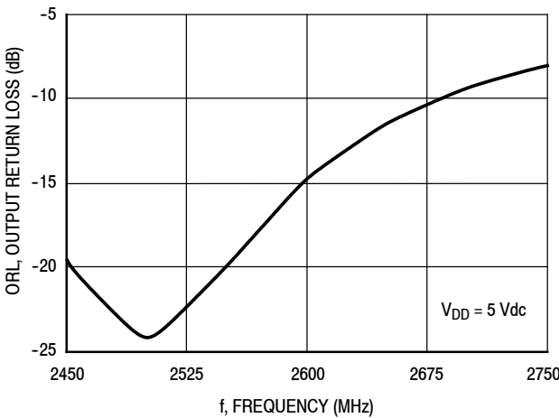
Figure 39. Output Return Loss (S22) versus Frequency
