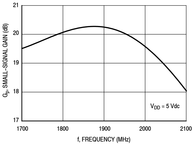
Figure 21. Small-Signal Gain (S21) versus Frequency
