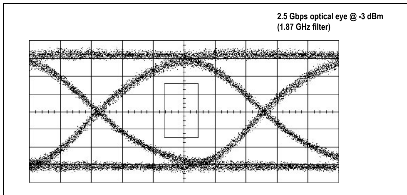
Figure 3-5. Typical Eye Diagram
