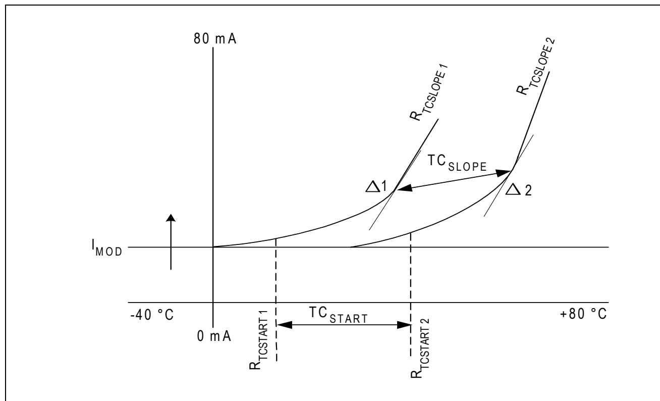
Figure 3-6. Temperature Compensation
