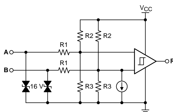
Figure 28. Receiver Inputs
