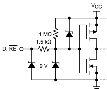
Figure 25. D and \overline{RE} Inputs
