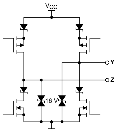
Figure 29. Driver Outputs
