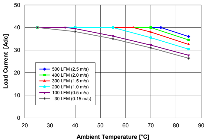
Fig. 1.5V.1: Available load current vs. ambient air temperature and airflow rates for QM48S40015 converter mounted vertically with air flowing from pin 3 to pin 1, MOSFET temperature \leq 120^\circ\text{C} , V_{in} = 48\text{ V} .
