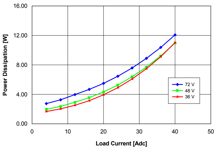
Fig. 2.0V.5: Power dissipation vs. load current and input voltage for converter mounted vertically with air flowing from pin 3 to pin 1 at a rate of 300 LFM (1.5 m/s) and Ta = 25°C.
