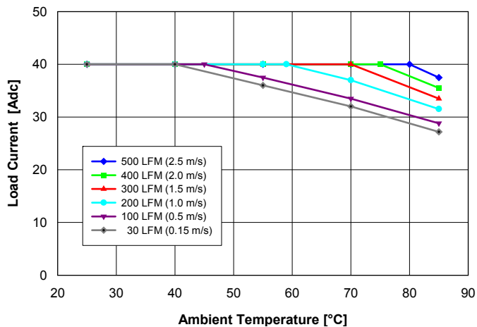
Fig. 1.2V.1: Available load current vs. ambient air temperature and airflow rates for QM48S40012 converter mounted vertically with air flowing from pin 3 to pin 1, MOSFET temperature \leq 120^\circ\text{C} , V_{in} = 48\text{ V} .
