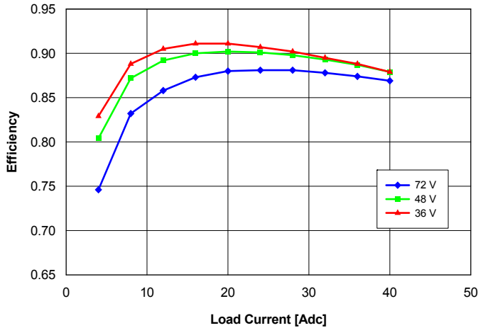
Fig. 2.0V.3: Efficiency vs. load current and input voltage for converter mounted vertically with air flowing from pin 3 to pin 1 at a rate of 300 LFM (1.5 m/s) and Ta = 25°C.
