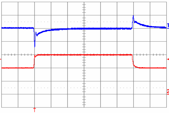
Fig. 3.3V.9: Output voltage response to load current step-change (20 A – 30 A – 20 A) at V_{in} = 48\text{ V} . Top trace: output voltage (100 mV/div.). Bottom trace: load current (10 A/div). Current slew rate: 1 A/ \mu\text{s} . C_o = 470\text{ }\mu\text{F} tantalum + 1 \mu\text{F} ceramic. Time scale: 0.2 ms/div.
