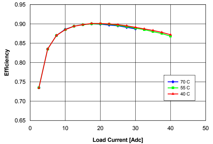
Fig. 2.0V.4: Efficiency vs. load current and ambient temperature for converter mounted vertically with Vin = 48 V and air flowing from pin 3 to pin 1 at a rate of 200 LFM (1.0 m/s).
