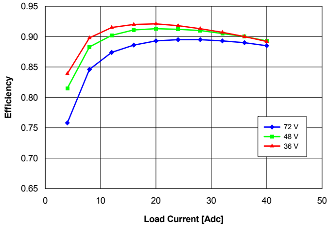
Fig. 2.5V.3: Efficiency vs. load current and input voltage for converter mounted vertically with air flowing from pin 3 to pin 1 at a rate of 300 LFM (1.5 m/s) and Ta = 25°C.
