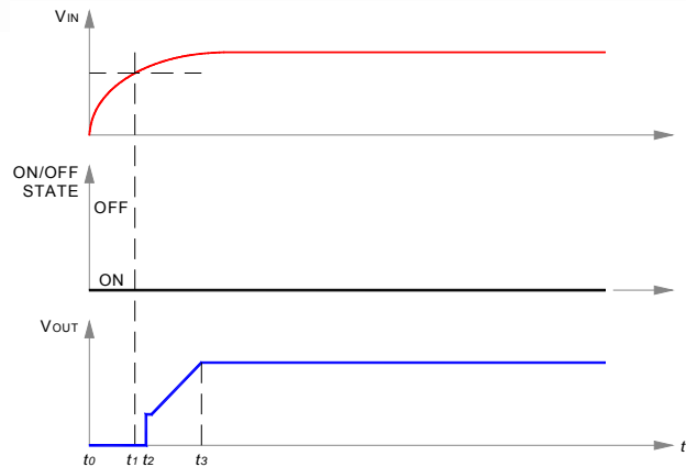
Fig. E: Start-up scenario #1.
