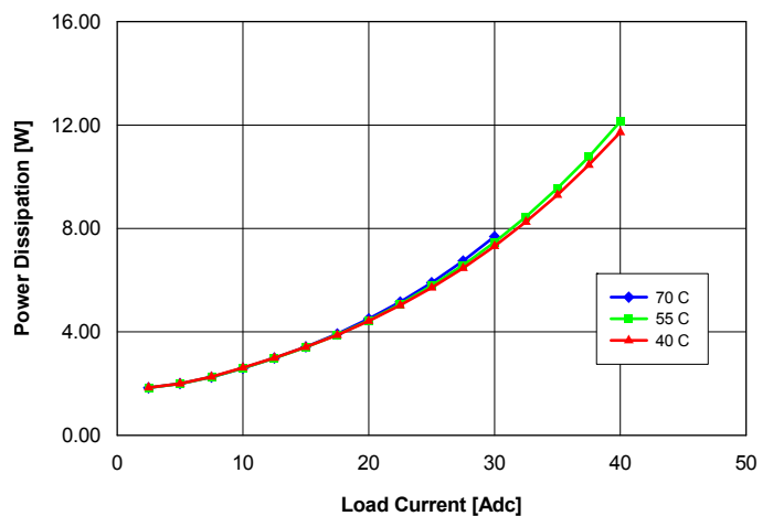
Fig. 2.0V.6: Power dissipation vs. load current and ambient temperature for converter mounted vertically with Vin = 48 V and air flowing from pin 3 to pin 1 at a rate of 200 LFM (1.0 m/s).
