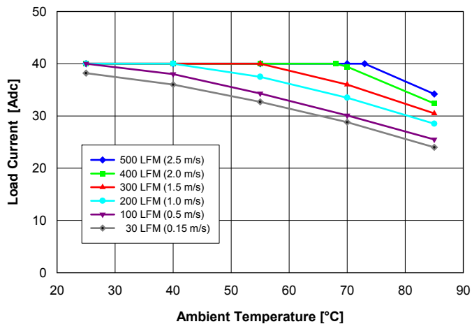
Fig. 2.0V.1: Available load current vs. ambient air temperature and airflow rates for QM48S40020 converter mounted vertically with air flowing from pin 3 to pin 1, MOSFET temperature \leq 120^\circ\text{C} , V_{in} = 48\text{ V} .
