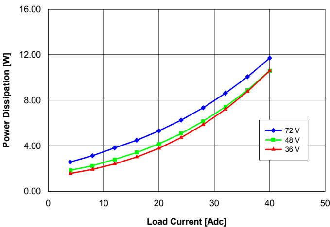
Fig. 1.8V.5: Power dissipation vs. load current and input voltage for converter mounted vertically with air flowing from pin 3 to pin 1 at a rate of 300 LFM (1.5 m/s) and T_a = 25^\circ\text{C} .
