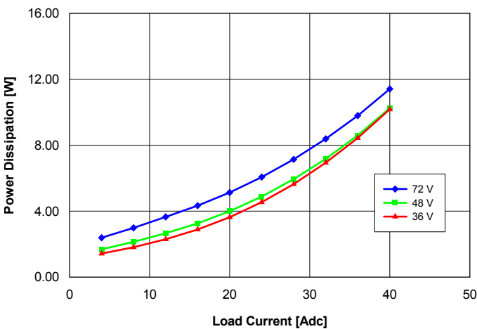
Fig. 1.5V.5: Power dissipation vs. load current and input voltage for converter mounted vertically with air flowing from pin 3 to pin 1 at a rate of 300 LFM (1.5 m/s) and T_a = 25^\circ\text{C} .
