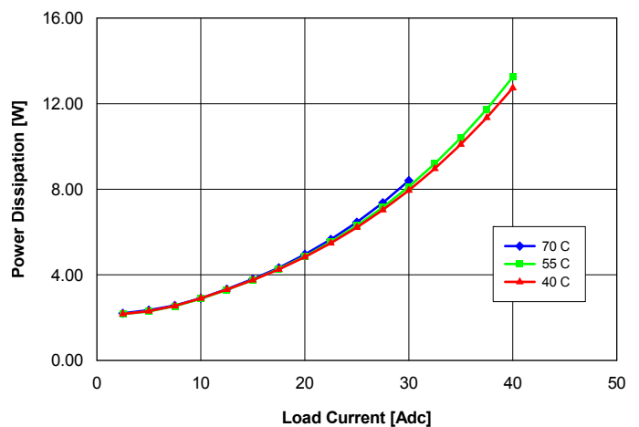
Fig. 2.5V.6: Power dissipation vs. load current and ambient temperature for converter mounted vertically with Vin = 48 V and air flowing from pin 3 to pin 1 at a rate of 200 LFM (1.0 m/s).
