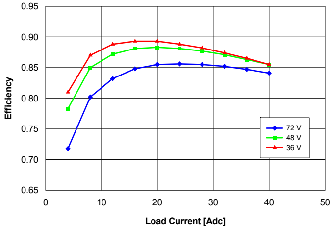
Fig. 1.5V.3: Efficiency vs. load current and input voltage for converter mounted vertically with air flowing from pin 3 to pin 1 at a rate of 300 LFM (1.5 m/s) and T_a = 25^\circ\text{C} .
