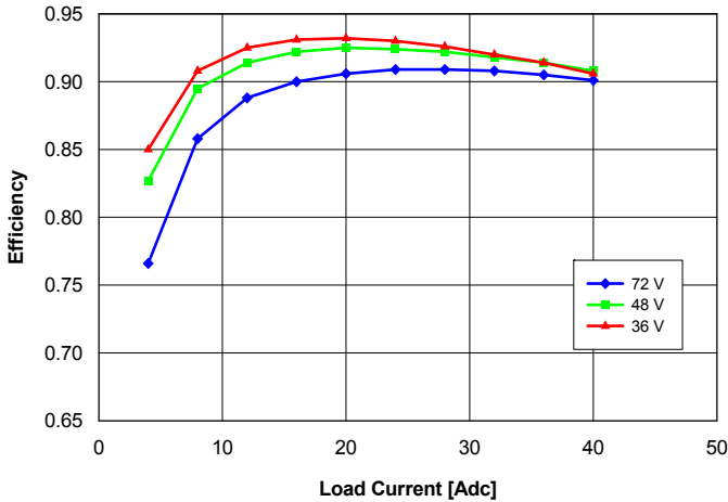
Fig. 3.3V.3: Efficiency vs. load current and input voltage for converter mounted vertically with air flowing from pin 3 to pin 1 at a rate of 300 LFM (1.5 m/s) and Ta = 25°C.
