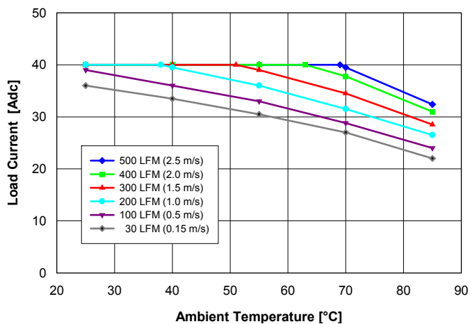
Fig. 2.5V.1: Available load current vs. ambient air temperature and airflow rates for QM48S40025 converter mounted vertically with air flowing from pin 3 to pin 1, MOSFET temperature \leq 120^\circ\text{C} , V_{in} = 48\text{ V} .
