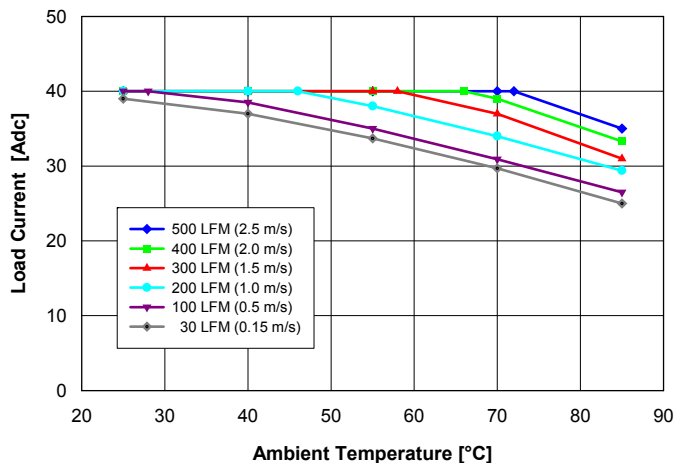
Fig. 1.8V.1: Available load current vs. ambient air temperature and airflow rates for QM48S40018 converter mounted vertically with air flowing from pin 3 to pin 1, MOSFET temperature \leq 120^\circ\text{C} , V_{in} = 48\text{ V} .
