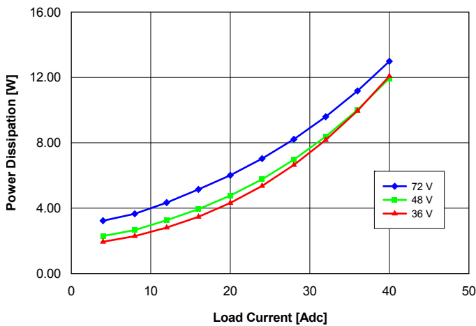
Fig. 2.5V.5: Power dissipation vs. load current and input voltage for converter mounted vertically with air flowing from pin 3 to pin 1 at a rate of 300 LFM (1.5 m/s) and Ta = 25°C.
