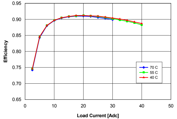
Fig. 2.5V.4: Efficiency vs. load current and ambient temperature for converter mounted vertically with Vin = 48 V and air flowing from pin 3 to pin 1 at a rate of 200 LFM (1.0 m/s).
