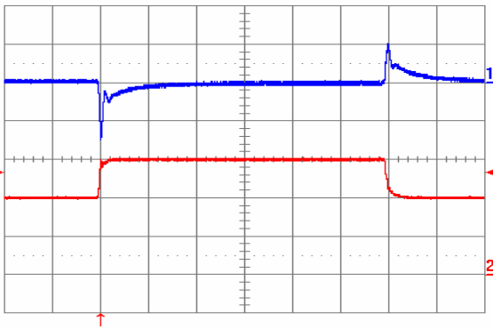
Fig. 2.0V.9: Output voltage response to load current step-change (20 A – 30 A – 20 A) at V_{in} = 48\text{ V} . Top trace: output voltage (100 mV/div.). Bottom trace: load current (10 A/div). Current slew rate: 1 A/ \mu\text{s} . C_o = 470\ \mu\text{F} tantalum + 1 \mu\text{F} ceramic. Time scale: 0.2 ms/div.
