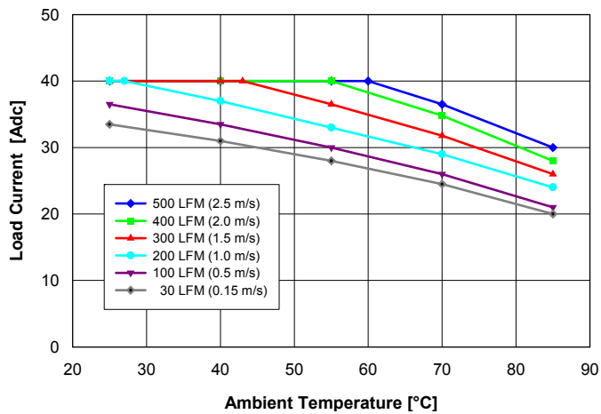
Fig. 3.3V.1: Available load current vs. ambient air temperature and airflow rates for QM48S40033 converter mounted vertically with air flowing from pin 3 to pin 1, MOSFET temperature \leq 120^\circ\text{C} , V_{in} = 48\text{ V} .
