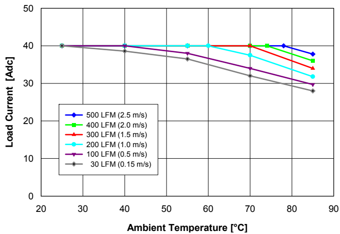
Fig. 1.0V.1: Available load current vs. ambient air temperature and airflow rates for QM48S40010 converter mounted vertically with air flowing from pin 3 to pin 1, MOSFET temperature \leq 120^\circ\text{C} , V_{in} = 48\text{ V} .
