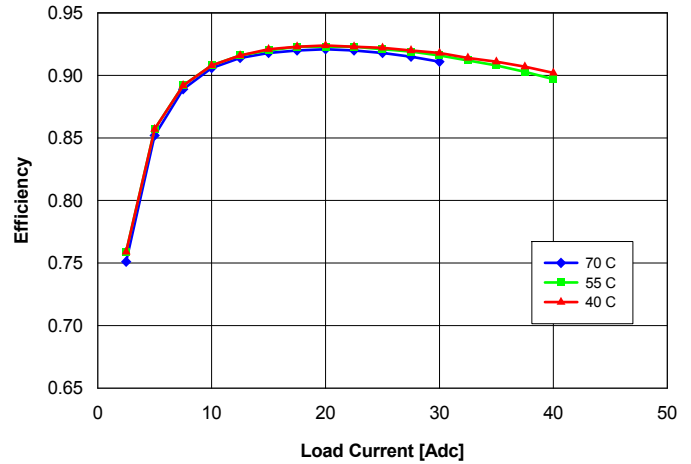
Fig. 3.3V.4: Efficiency vs. load current and ambient temperature for converter mounted vertically with Vin = 48 V and air flowing from pin 3 to pin 1 at a rate of 200 LFM (1.0 m/s).
