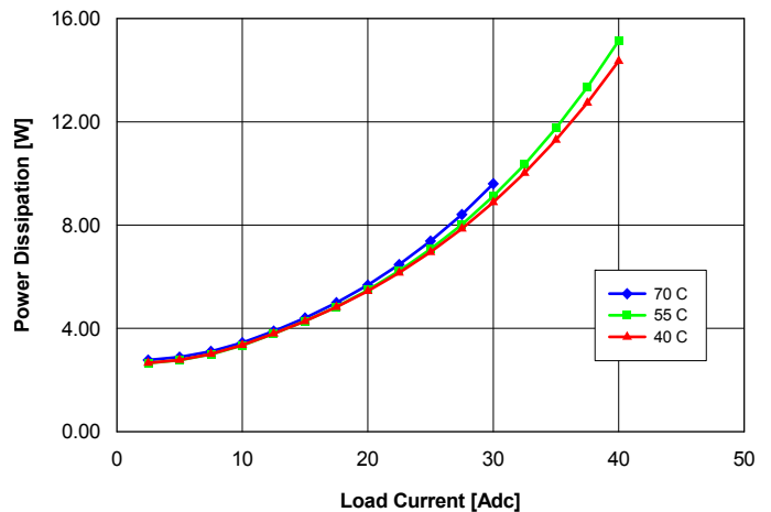
Fig. 3.3V.6: Power dissipation vs. load current and ambient temperature for converter mounted vertically with Vin = 48 V and air flowing from pin 3 to pin 1 at a rate of 200 LFM (1.0 m/s).
