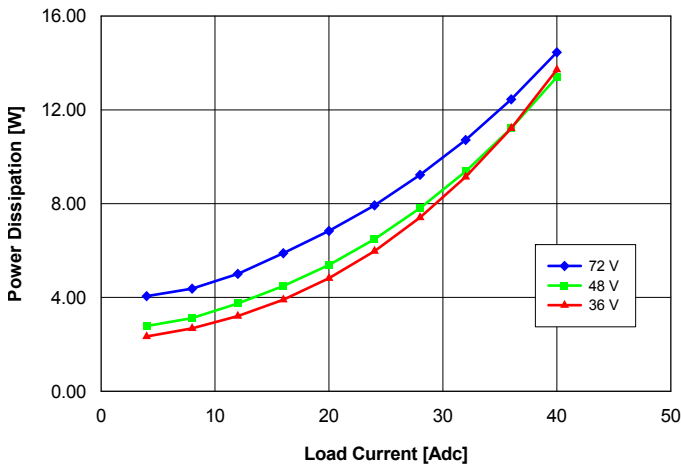
Fig. 3.3V.5: Power dissipation vs. load current and input voltage for converter mounted vertically with air flowing from pin 3 to pin 1 at a rate of 300 LFM (1.5 m/s) and Ta = 25°C.
