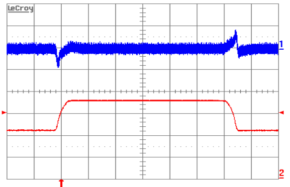
Figure 8. Output voltage response to load current step (12.5A–18.75A–12.5A) at V_{in}=48\text{V} . Top trace: output voltage (50 mV/div.). Bottom trace: load current (5A/div.). Current slew rate: 0.1A/ \mu\text{s} . C_o=1\mu\text{F} ceramic + 10 \mu\text{F} tantalum. Time scale: 0.2ms/div.
