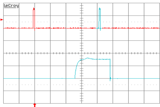
Figure 14. Load current (top trace, 20 A/div., 50 ms/div.) into a 10 m \Omega short circuit during restart, at V_{in} = 48 \text{ V} . Bottom trace (20 A/div., 2 ms/div.) is an expansion of the on-time portion of the top trace
