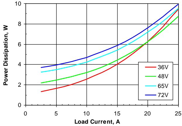
Figure 4. Power dissipation vs. load current and input voltage for SSQE48T25033 converter mounted vertically with air flowing from pin 1 to pin 3at a rate of 300 LFM (1.5 m/s) and T_a = 25\text{ }^\circ\text{C} .
