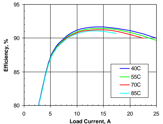
Figure 3. Efficiency vs. load current and ambient temperature for SSQE48T25033 converter mounted vertically with Vin=48V and air flowing from pin 1 to pin 3 at a rate of 200LFM (1.0m/s).
