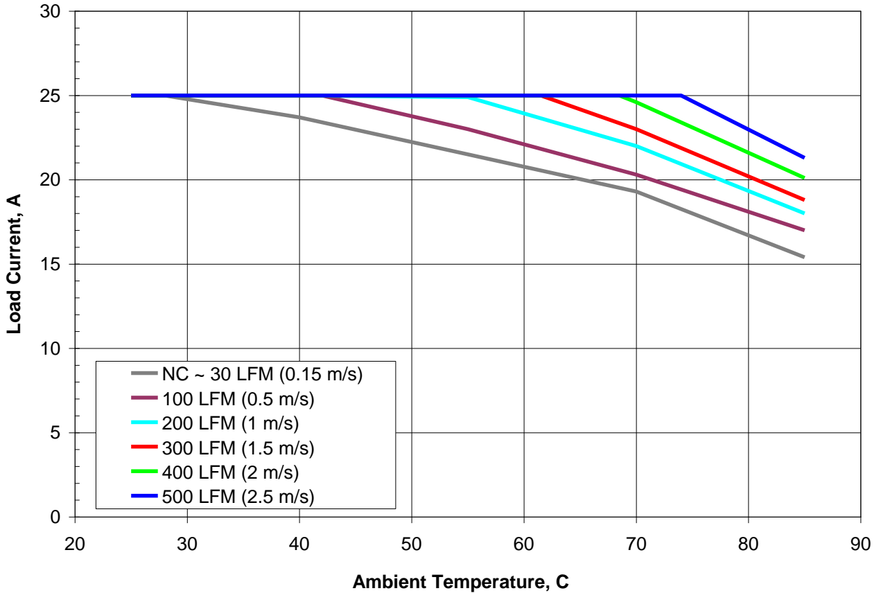
Figure 1. Available load current vs. ambient air temperature and airflow rates for SSQE48T25033 converter mounted vertically with air flowing from pin 1 to pin 3, Vin = 48 V. Note: NC – Natural convection
