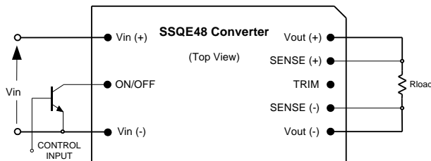
Fig. A: Circuit configuration for ON/OFF function.
