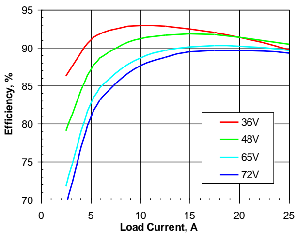
Figure 2. Efficiency vs. load current and input voltage for SSQE48T25033 converter mounted vertically with air flowing from pin 1 to pin 3 at a rate of 300 LFM (1.5 m/s) and Ta=25°C.
