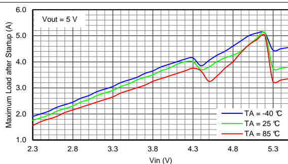
Figure 13. Maximum Load Current after Startup
