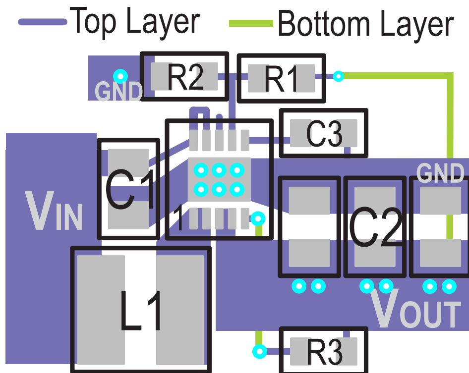
Figure 37. Layout Recommendation
