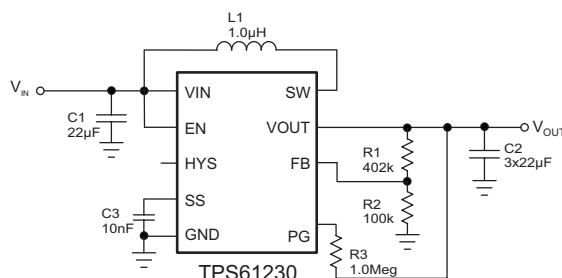
Figure 12. TPS61230 5-V Output Typical Application
