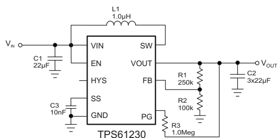
Figure 25. TPS61230 3.5-V Output Typical Application
