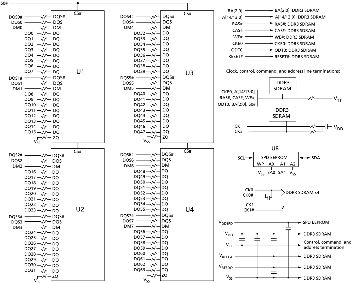
Figure 2: Functional Block Diagram (PCB 0698, R/C-C)
