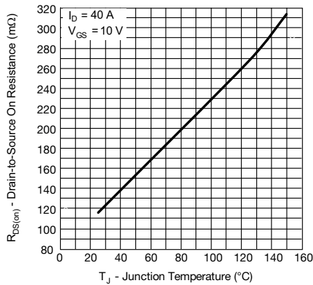
Fig. 6 - Normalized On-Resistance vs. Temperature
