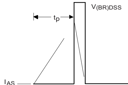
Fig. 20 - Unclamped Inductive Waveforms
