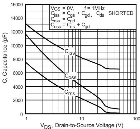
Fig. 14 - Typical Capacitance vs. Drain to Source Voltage
