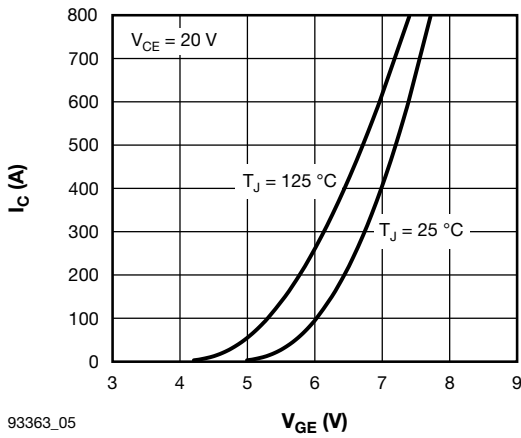
Fig. 5 - Typical IGBT Transfer Characteristics
