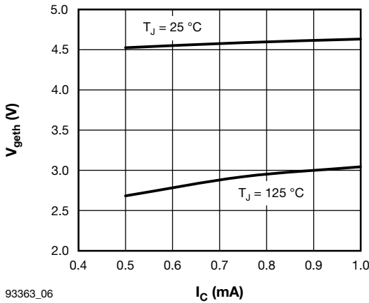
Fig. 6 - Typical IGBT Gate Threshold Voltage
